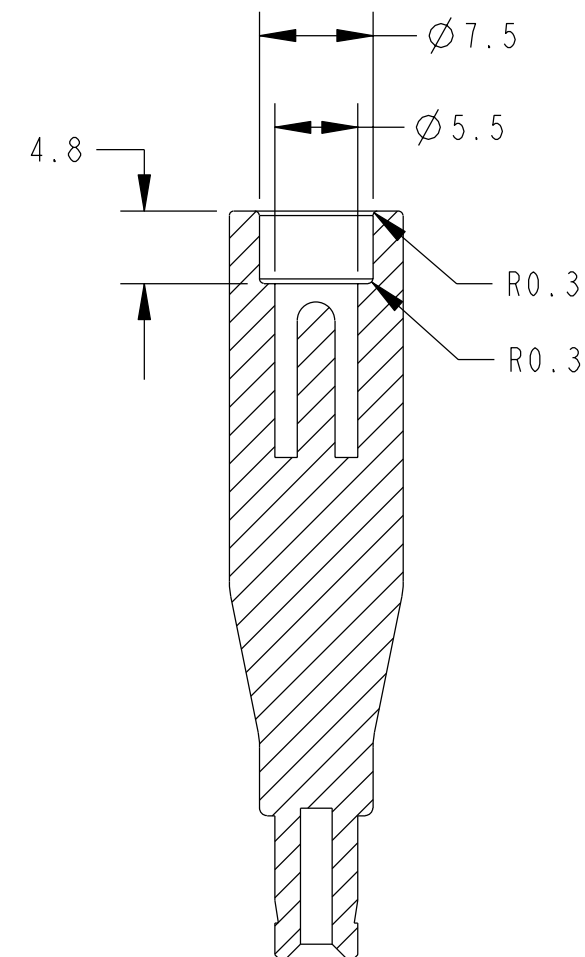
SECTION B-B
