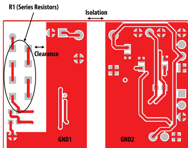
Figure 33. Bottom Layer Layout Recommendation
