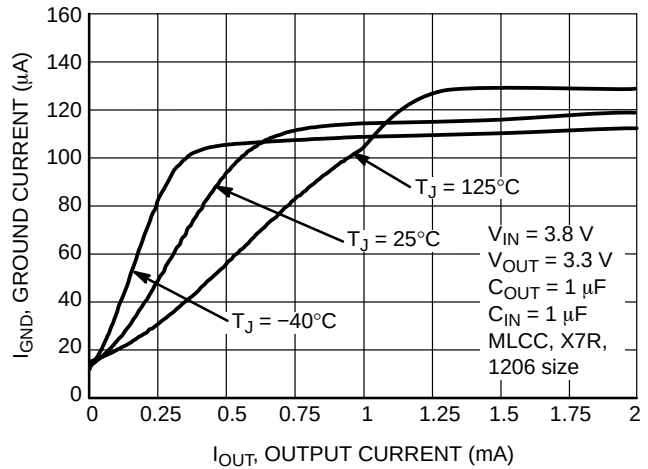
Figure 12. Ground Current vs. Output Current 0 mA to 2 mA at Temperature
