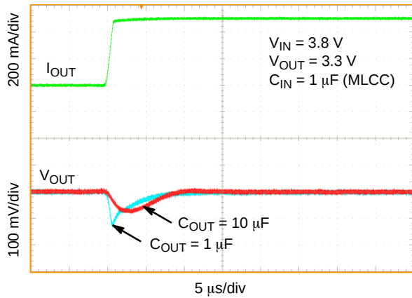
Figure 56. Load Transient Response – Rising Edge, V_{OUT} = 3.3 V, I_{OUT} = 1 mA to 500 mA, C_{OUT} = 1 μF, 10 μF
