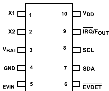
ISL1209 (10 LD MSOP) TOP VIEW
