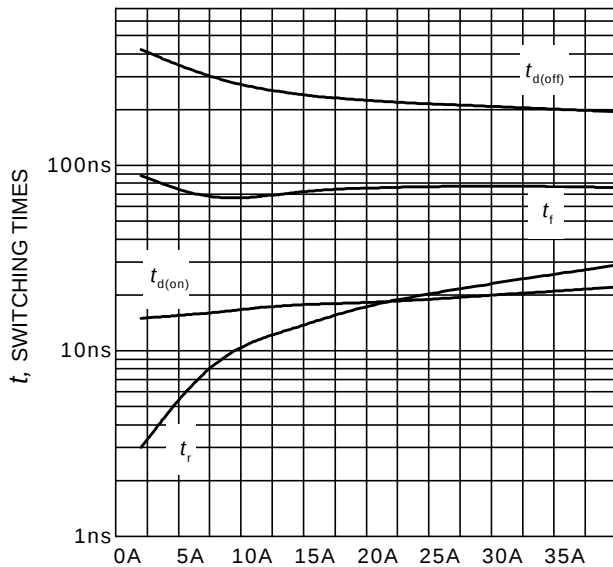
Figure 9. Typical switching times as a function of collector current (inductive load, T_J = 175^\circ\text{C} , V_{CE} = 400\text{V} , V_{GE} = 0/15\text{V} , r_G = 12\Omega , Dynamic test circuit in Figure E)
