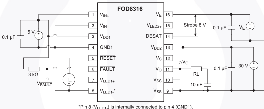
Figure 44. Reset Delay ( t_{RESET(FAULT)} ) Test Circuit
