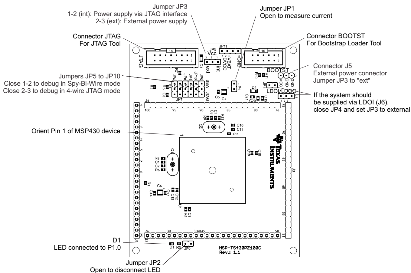
Figure B-58. MSP-TS430PZ100C Target Socket Module, PCB
