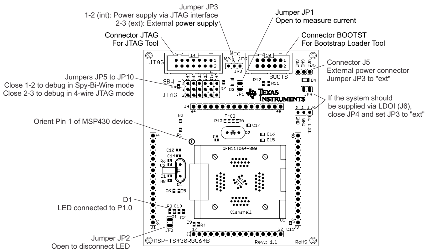
Figure B-40. MSP-TS430RGC64B Target Socket Module, PCB
