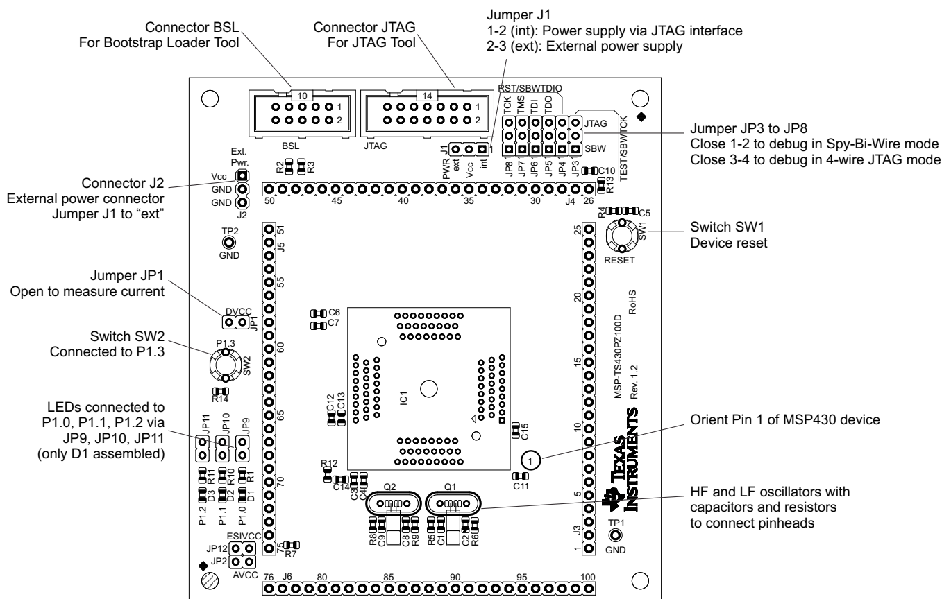
Figure B-60. MSP-TS430PZ100D Target Socket Module, PCB
