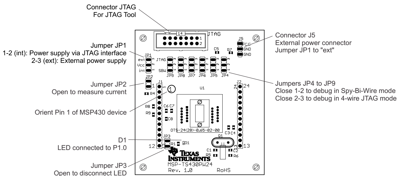
Figure B-10. MSP-TS430PW24 Target Socket Module, PCB
