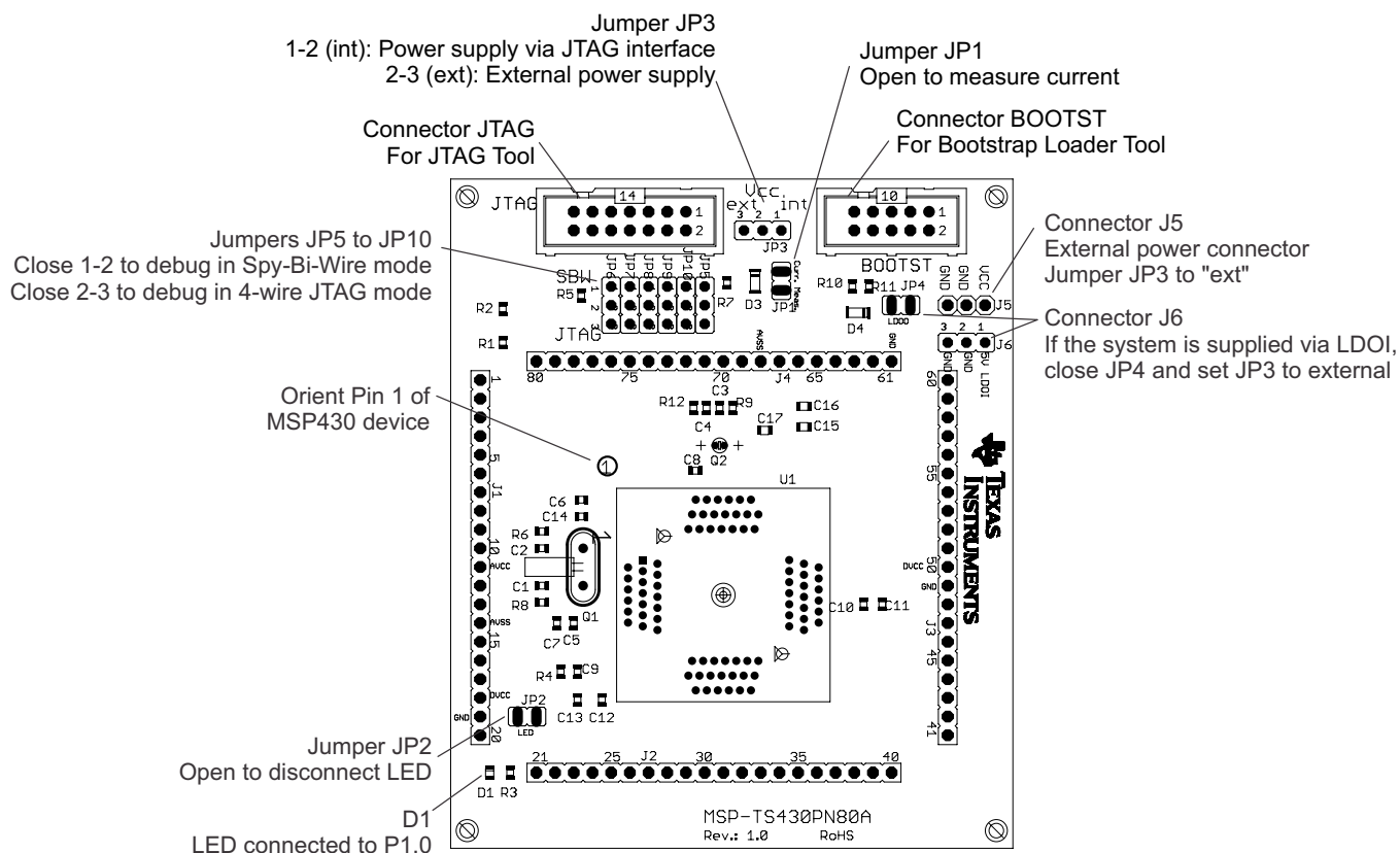
Figure B-48. MSP-TS430PN80A Target Socket Module, PCB
