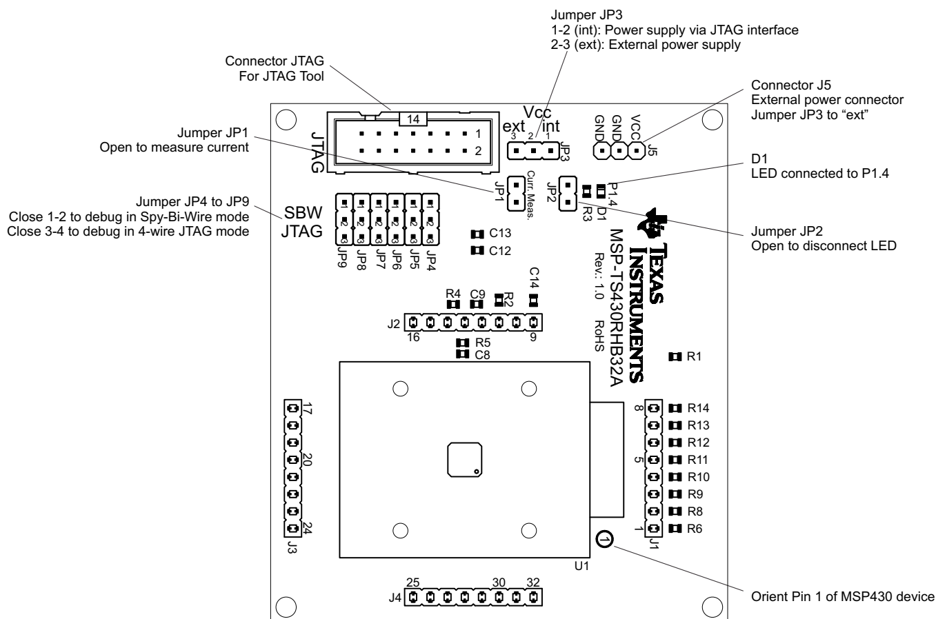
Figure B-18. MSP-TS430RHB32A Target Socket Module, PCB
