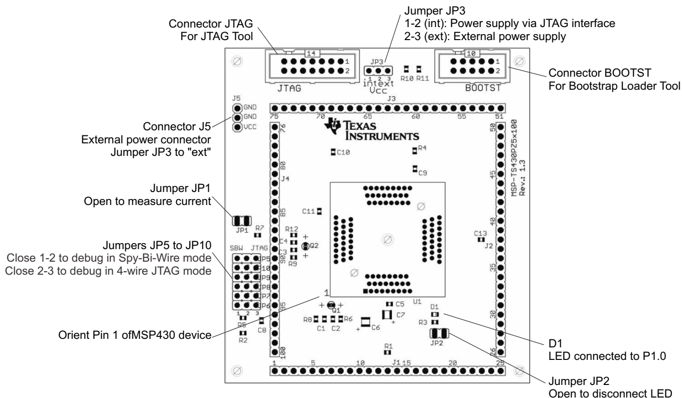
Figure B-62. MSP-TS430PZ5x100 Target Socket Module, PCB
