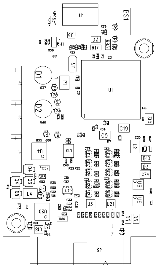
Figure B-80. MSP-FET USB Debugger, PCB (Top)
