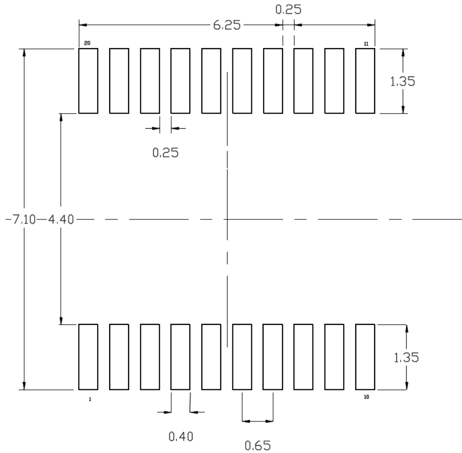
Figure 8.6 TSSOP Footprint (dimensions in millimeters)
