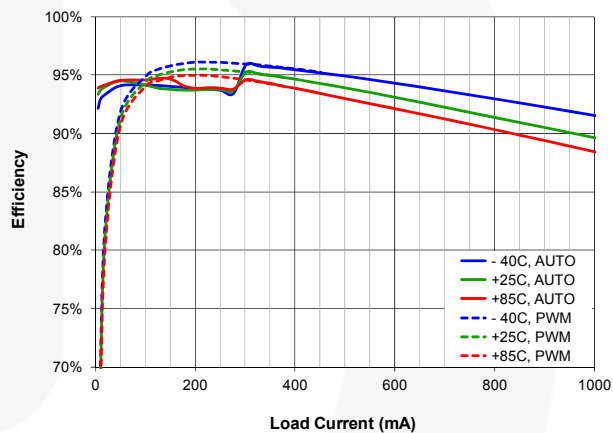
Figure 7. Efficiency vs. Load Current and Temperature, V_{OUT}=2.9 V, Dotted for FPWM
