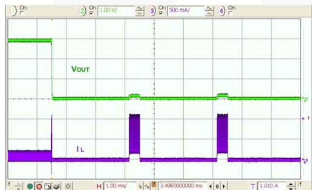
Figure 28. 250 m \Omega Fault, Rapid Fault, V_{OUT}=2.9 V, FAN53600
