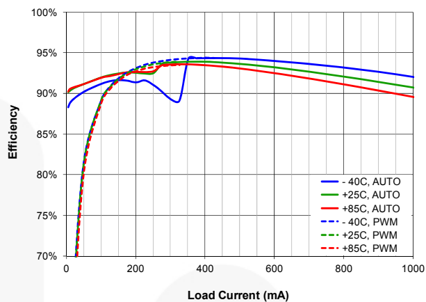
Figure 5. Efficiency vs. Load Current and Temperature V_{IN}=5 V, V_{OUT}=3.3 V, Dotted for FPWM
