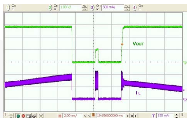
Figure 27. Over-Current, Load Increasing Past Current Limit, V_{OUT}=2.9 V, FAN53600
