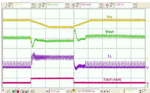
Figure 24. Combined Line / Load Transient, V_{OUT}=2.9\text{ V} , 3.9-3.3-3.9 V_{IN} , 10 \mu\text{s} Edge, 58-500-58 mA Load, 100 ns Edge
