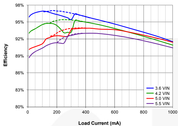
Figure 4. Efficiency vs. Load Current and Input Voltage, V_{OUT}=3.3 V, Dotted for Decreasing Load
