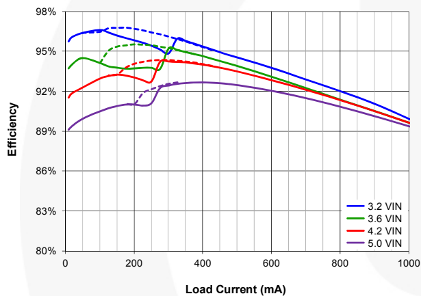
Figure 6. Efficiency vs. Load Current and Input Voltage, V_{OUT}=2.9 V, Dotted for Decreasing Load
