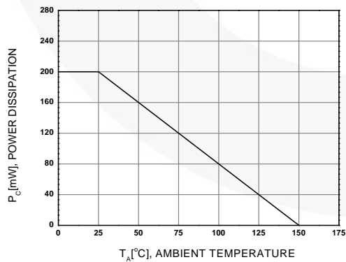
Figure 5. Power Derating
