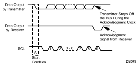
Figure 23-4. ACCESS.bus Acknowledge Cycle
