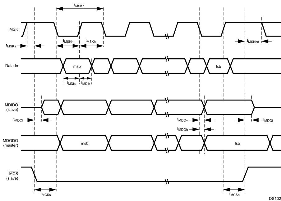
Figure 29-12. Microwire Transaction Timing, Normal Mode, SCIDL = 1
