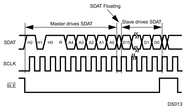
Figure 15-4. Serial Interface Read Timing
