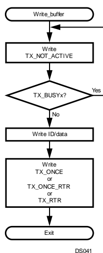
Figure 18-24. Buffer Write Routine
