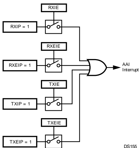
Figure 19-6. AAI Interrupt Structure
