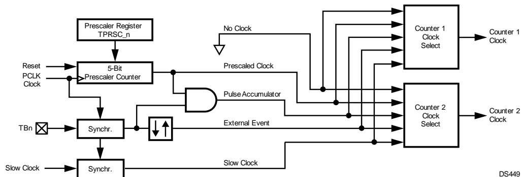
Figure 25-2. Multi-Function Timer Clock Source
