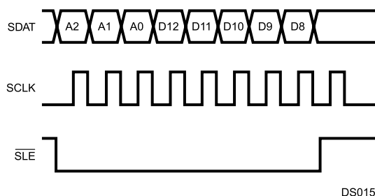
Figure 15-6. Serial Interface 8-bit Fast-Write Timing
