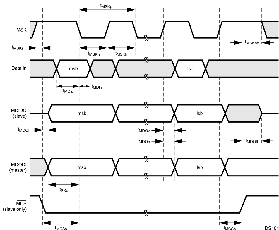
Figure 29-14. Microwire Transaction Timing, Alternate Mode, SCIDL = 1
