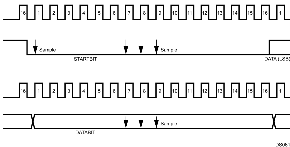
Figure 21-2. UART Asynchronous Communication
