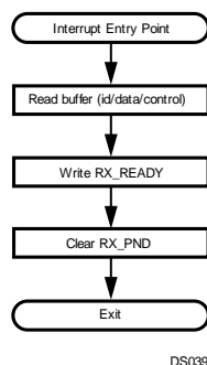
Figure 18-22. Buffer Read Routine (BUFFLOCK Enabled)
