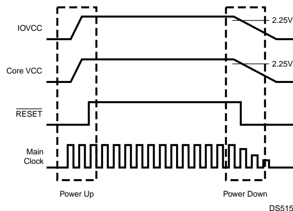
Figure 11-4. Power-On Reset Timing
