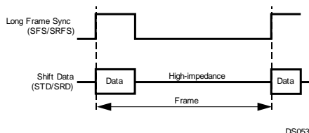
Figure 19-1. Normal Mode Frame
