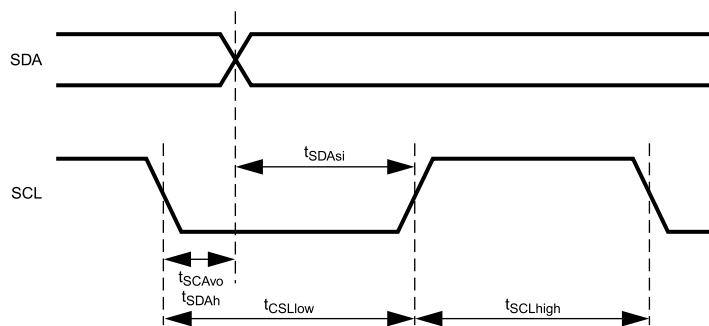
Figure 29-18. ACB Start Condition Timing
