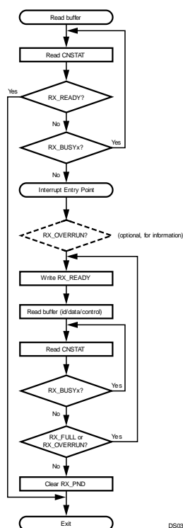
Figure 18-21. Buffer Read Routine (BUFFLOCK Disabled)
