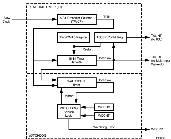
Figure 24-1. Timing and Watchdog Module Block Diagram
