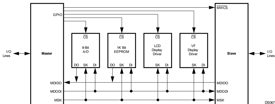
Figure 22-1. Microwire Interface
