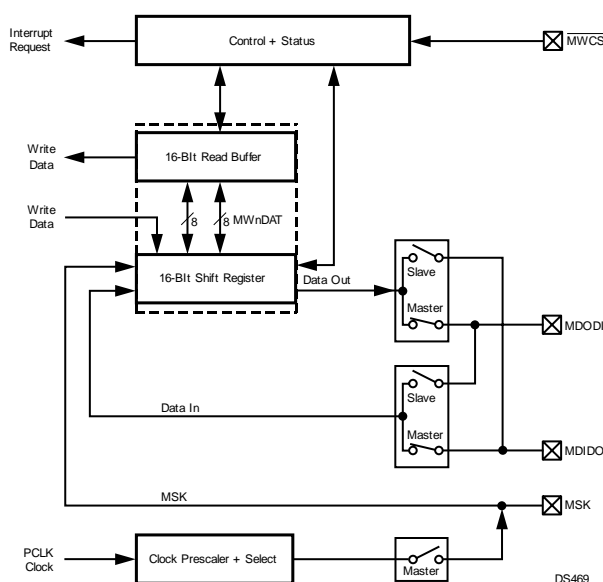
Figure 22-2. Microwire Block Diagram
