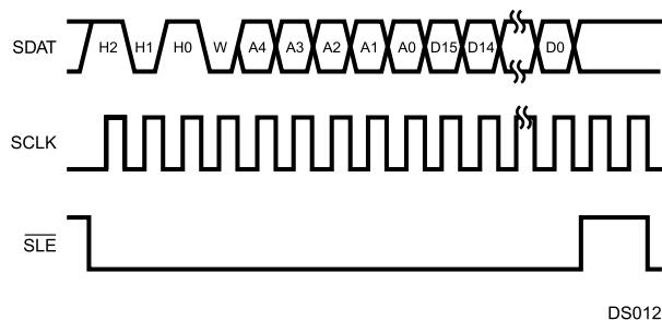
Figure 15-3. Serial Interface Write Timing
