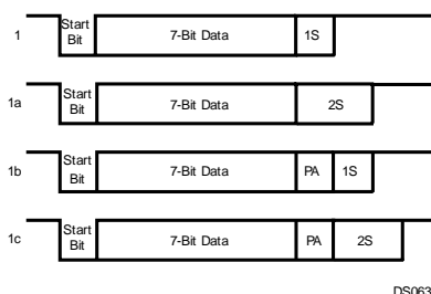
Figure 21-4. 7-Bit Data Frame Options
