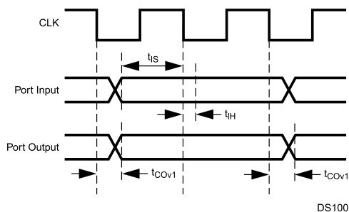
Figure 29-6. I/O Port Timing
