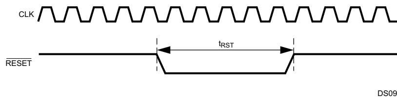
Figure 29-3. Non-Power-On Reset
