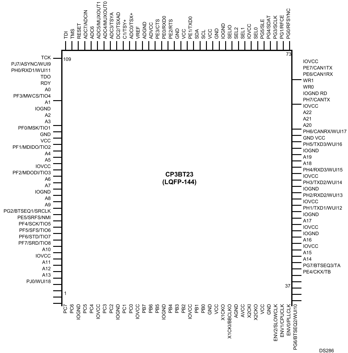
Figure 30-2. CP3BT23 in the LQFP-144 Package (Top View)
