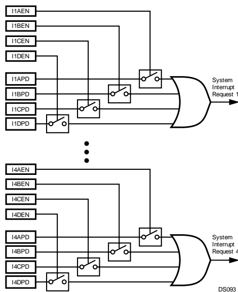
Figure 26-6. VTU Interrupt Request Structure
