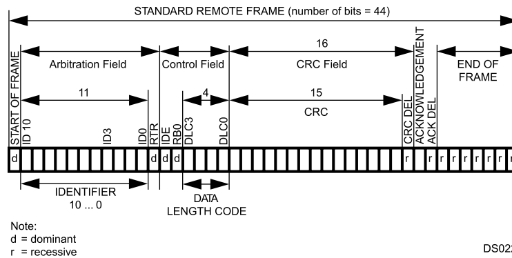
Figure 18-5. Standard Remote Frame
