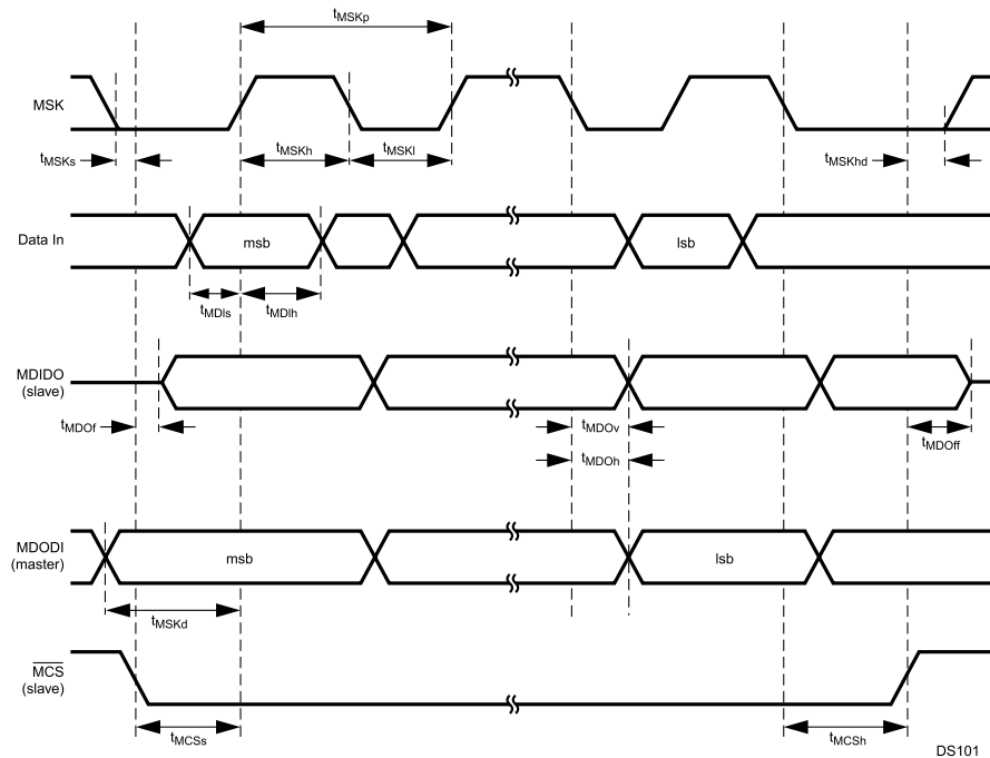
Figure 29-11. Microwire Transaction Timing, Normal Mode, SCIDL = 0
