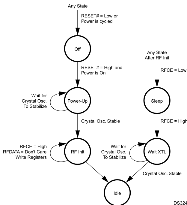
Figure 15-10. LMX5252 Power States
