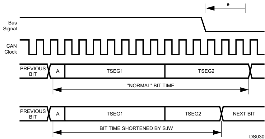
Figure 18-13. Resynchronization ( e < -\text{SJW} )
