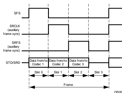
Figure 19-5. Accessing Three Devices in Network Mode
