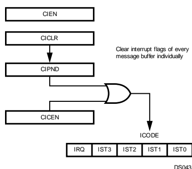
Figure 18-26. Interrupt Management
