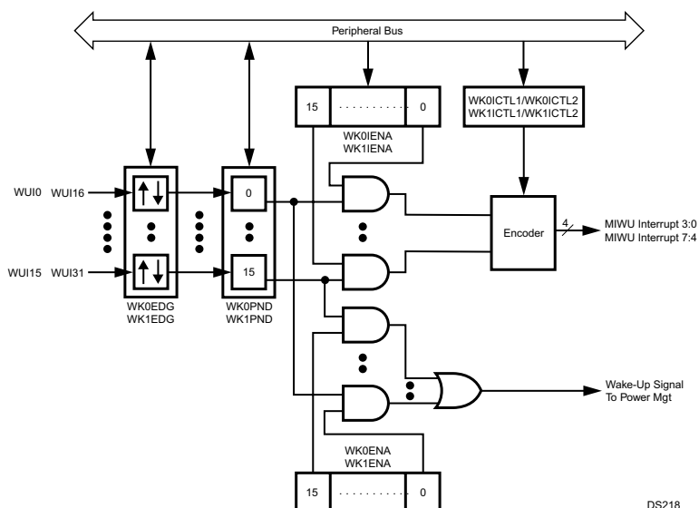
Figure 13-1. Multi-Input Wake-Up Module Block Diagram
