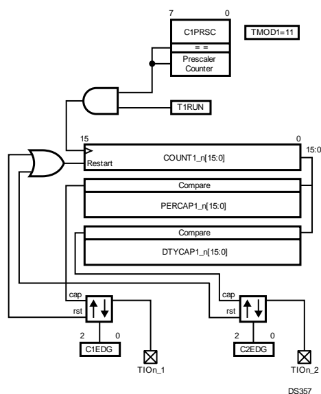
Figure 26-5. VTU Dual 16-bit Capture Mode
