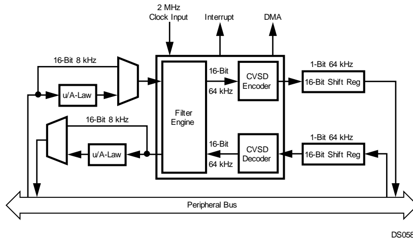
Figure 20-1. CVSD/PCM Converter Block Diagram
