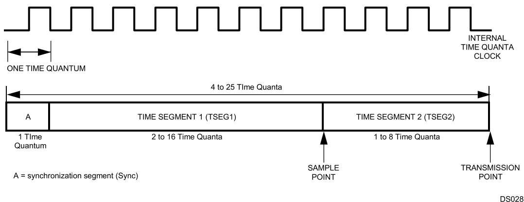
Figure 18-11. Bit Timing
