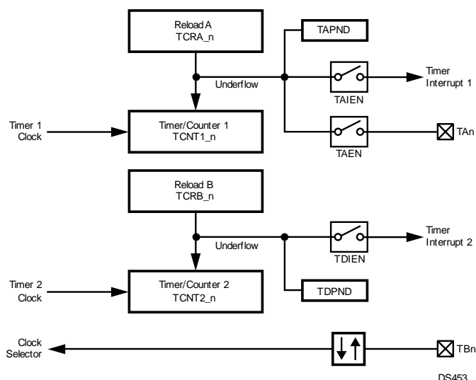
Figure 25-6. Dual-Independent Timer/Counter Mode
