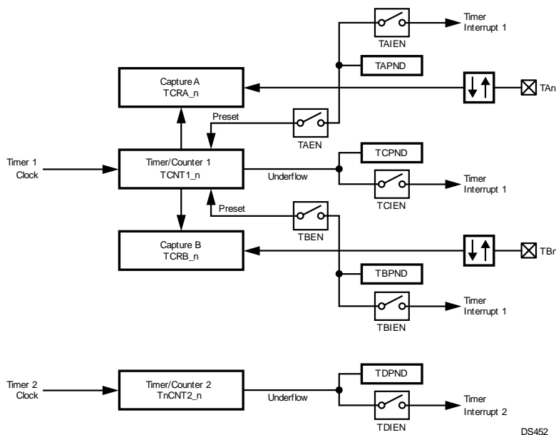
Figure 25-5. Dual-Input Capture Mode
