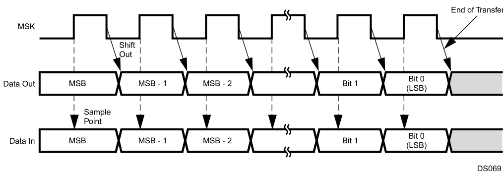
Figure 22-3. Normal Mode (SCIDL = 0)
