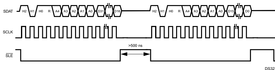
Figure 15-8. 32-Bit Read Timing
