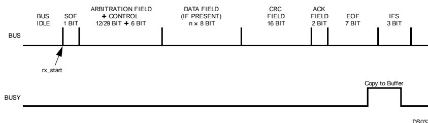
Figure 18-20. Receive Timing
