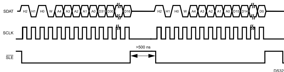
Figure 15-7. 32-Bit Write Timing
