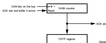
Figure 18-27. Time Stamp Counter
