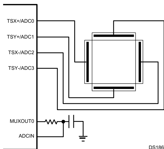
Figure 16-2. Touchscreen Interface
