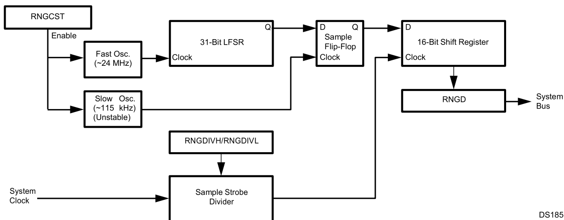
Figure 17-1. RNG Module Block Diagram
