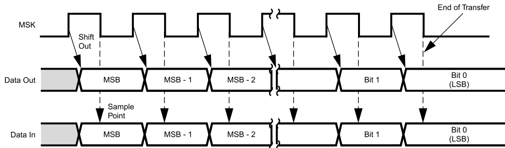
Figure 22-5. Alternate Mode (SCIDL = 0)
