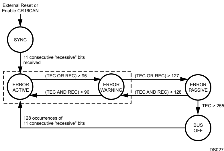
Figure 18-10. Bus States
