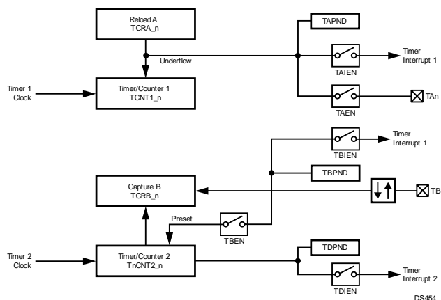
Figure 25-7. Input Capture Plus Timer Mode
