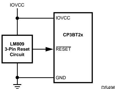
Figure 11-5. Simple External Reset
