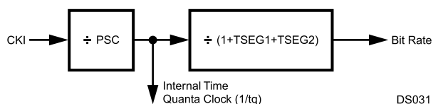
Figure 18-14. CAN Prescaler
