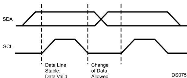
Figure 23-1. Bit Transfer
