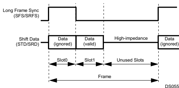
Figure 19-3. Network Mode Frame
