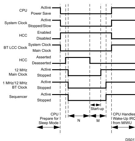
Figure 15-12. Bluetooth Sleep Mode Sequence
