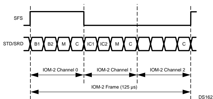
Figure 19-9. IOM-2 Frame Structure
