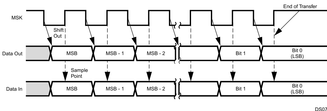
Figure 22-4. Normal Mode (SCIDL = 1)
