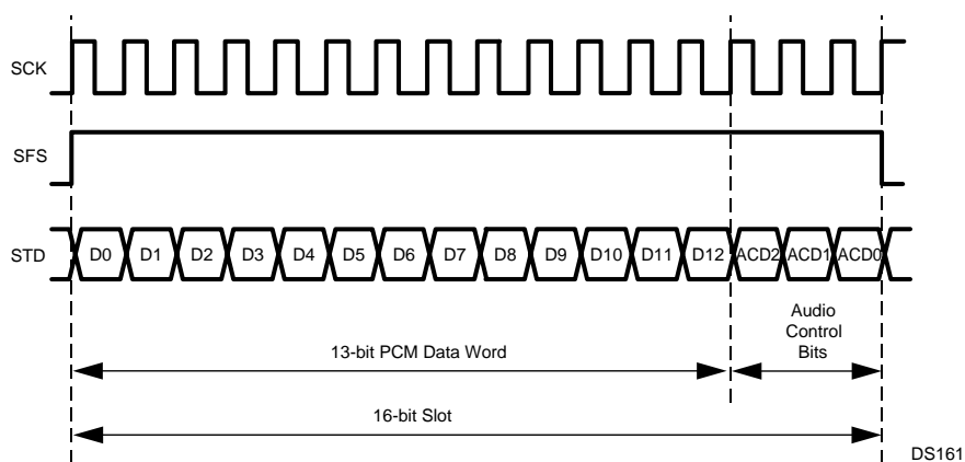
Figure 19-8. Audio Slot with Audio Control Data
