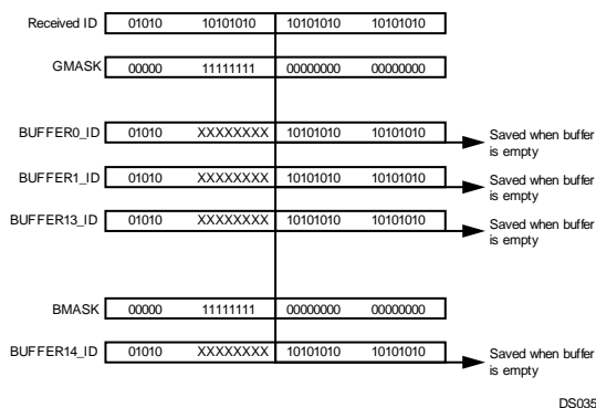
Figure 18-18. Message Storage with BUFFLOCK Enabled
