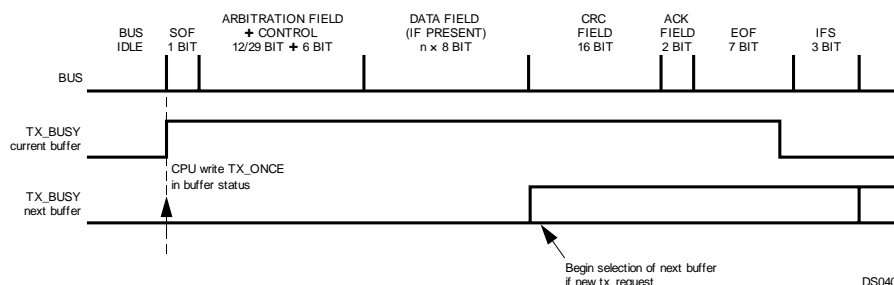
Figure 18-23. Data Transmission
