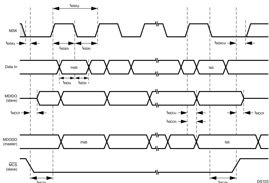
Figure 29-13. Microwire Transaction Timing, Alternate Mode, SCIDL = 0
