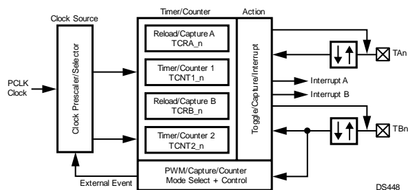
Figure 25-1. Multi-Function Timer Block Diagram
