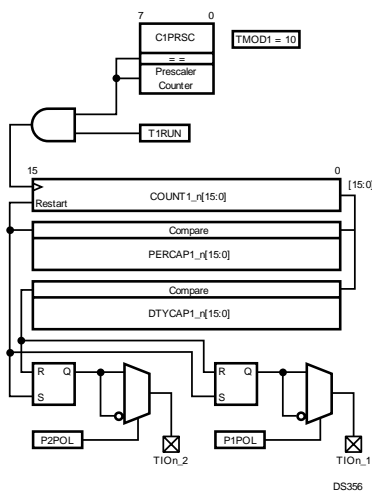
Figure 26-4. VTU 16-bit PWM Mode
