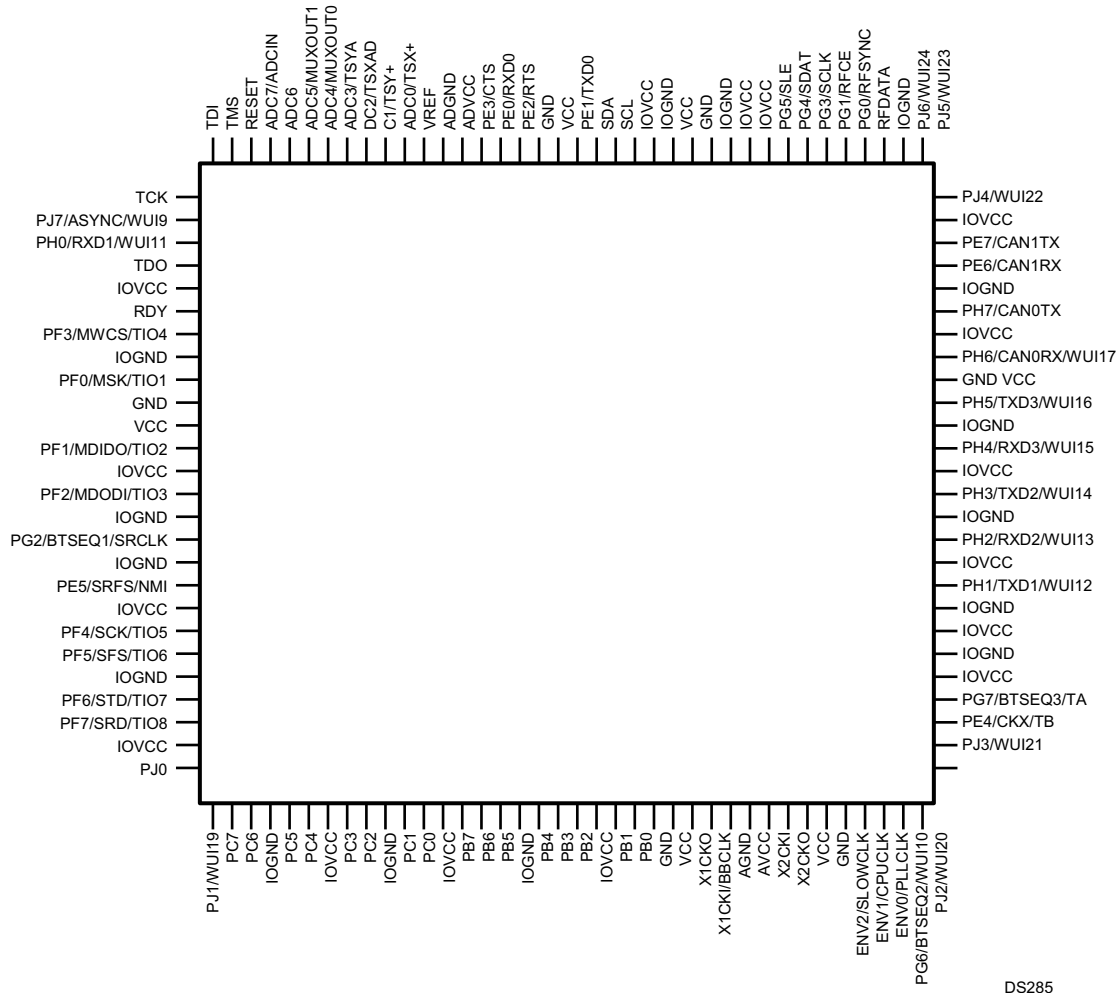
Figure 30-1. CP3BT23 in the LQFP-128 Package (Top View)
