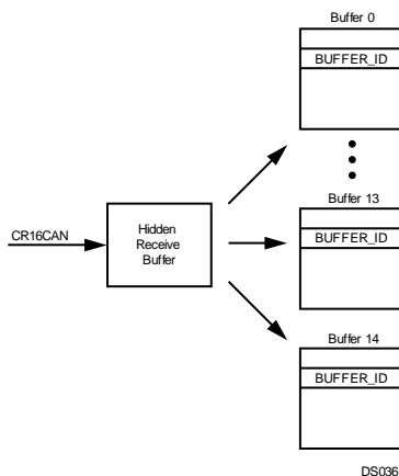
Figure 18-19. Receive Buffer
