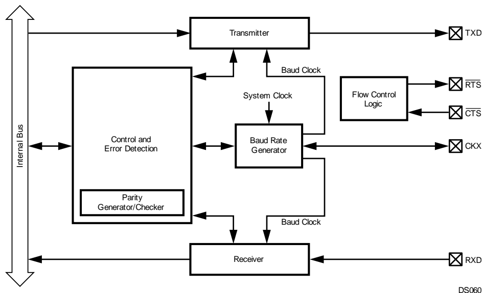
Figure 21-1. UART Block Diagram
