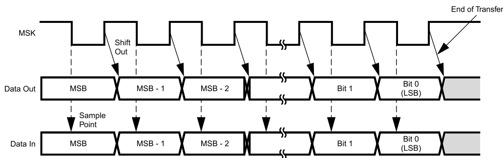
Figure 22-5. Alternate Mode (SCIDL = 0)
