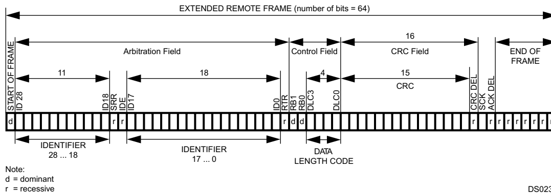
Figure 18-6. Extended Remote Frame
