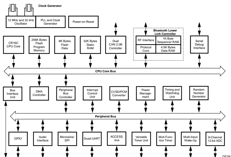
Figure 1-1. Block Diagram
