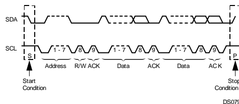
Figure 23-5. A Complete ACCESS.bus Data Transaction
