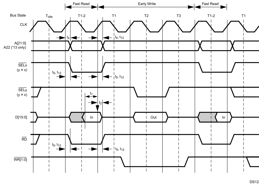
Figure 29-26. Early Write Between Fast Read Cycles
