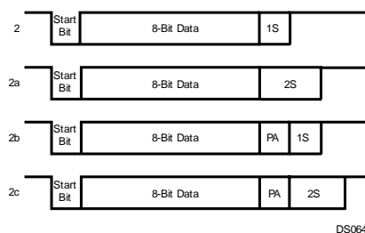
Figure 21-5. 8-Bit Data Frame Options
