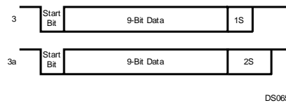
Figure 21-6. 9-bit Data Frame Options
