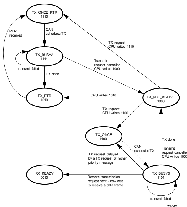
Figure 18-25. Transmit Buffer States
