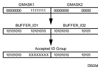
Figure 18-17. Acceptance of a Group of Identifiers
