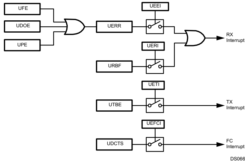
Figure 21-7. UART Interrupts
