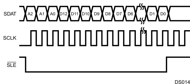
Figure 15-5. Serial Interface 16-bit Fast-Write Timing
