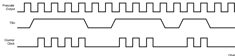
Figure 25-3. Pulse-Accumulate Mode
