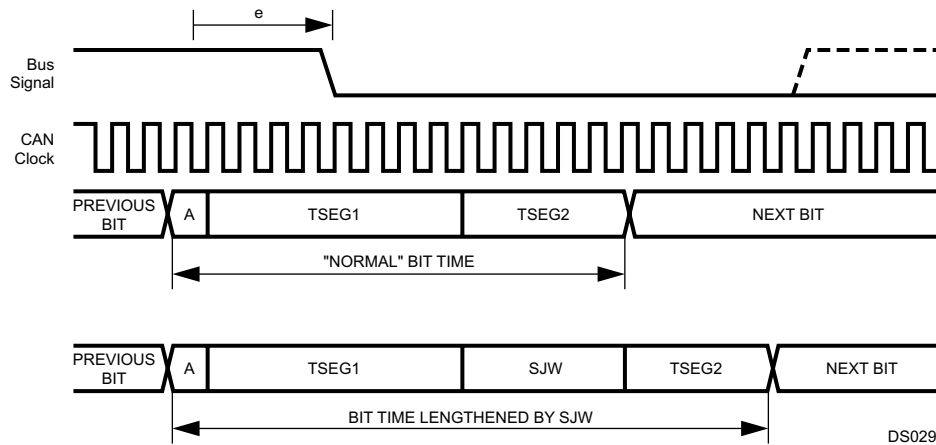
Figure 18-12. Resynchronization ( e > \text{SJW} )
