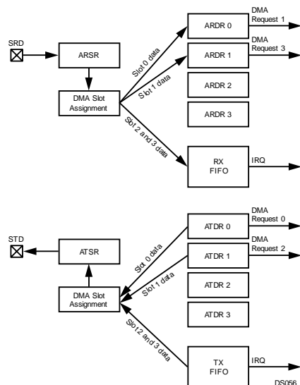
Figure 19-4. IRQ/DMA Support in Network Mode
