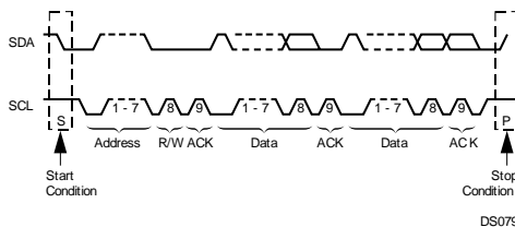
Figure 23-3. ACCESS.bus Data Transaction
