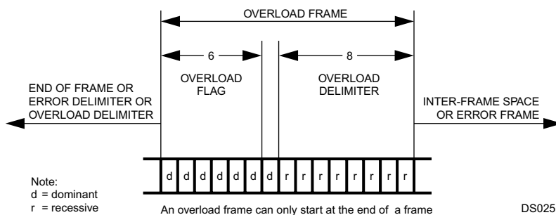
Figure 18-8. Overload Frame
