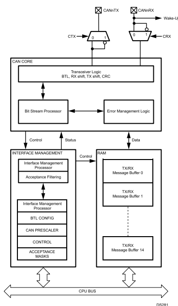
Figure 18-1. CAN Block Diagram
