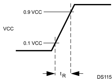
Figure 29-4. Power-On Reset
