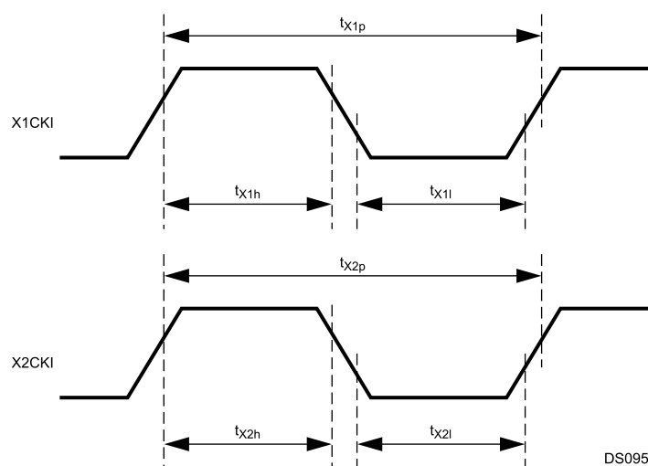
Figure 29-1. Clock Timing
