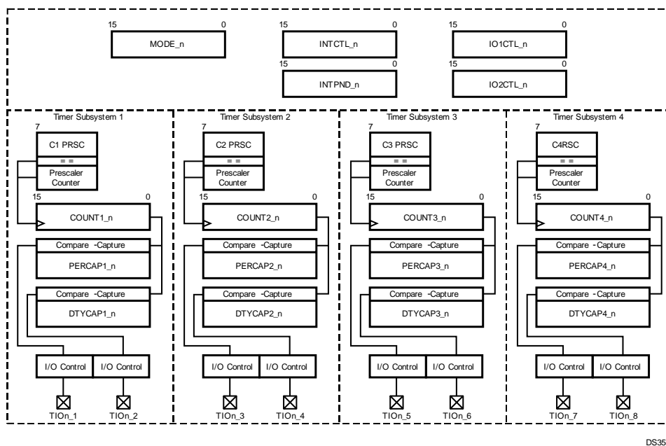
Figure 26-1. Versatile Timer Unit Block Diagram
