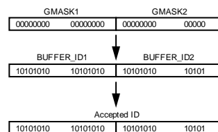
Figure 18-16. Acceptance of a Single Identifier
