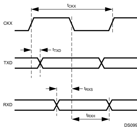
Figure 29-5. UART Synchronous Mode Timing
