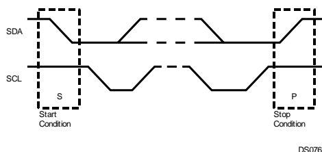
Figure 23-2. Start and Stop Conditions
