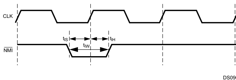
Figure 29-2. \overline{\text{NMI}} Signal Timing
