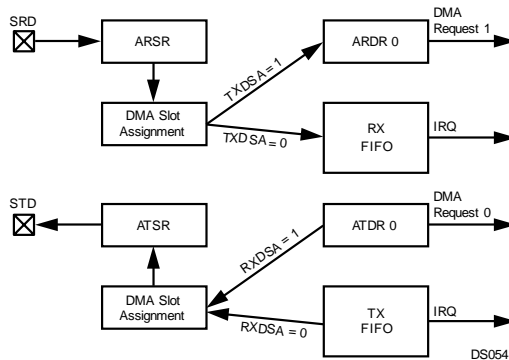
Figure 19-2. IRQ/DMA Support in Normal Mode
