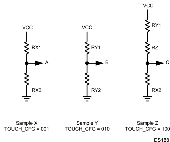
Figure 16-4. Touchscreen Driver Modes
