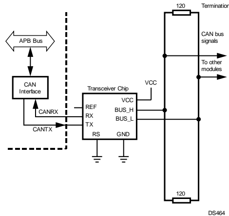
Figure 18-31. External Transceiver
