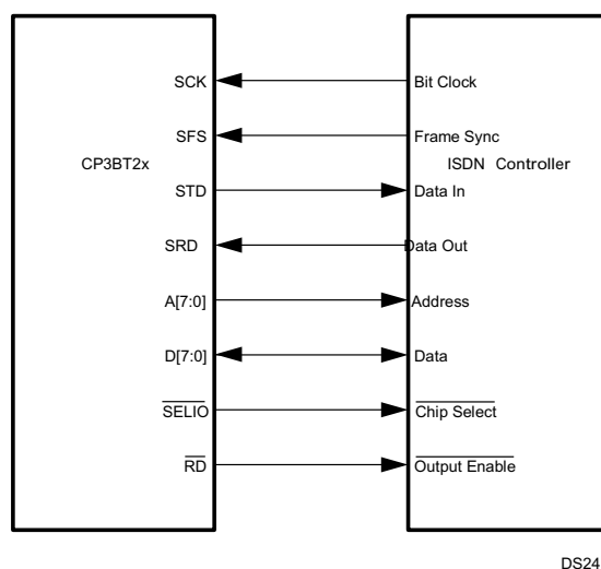
Figure 19-10. CP3BT23/ISDN Controller Connections
