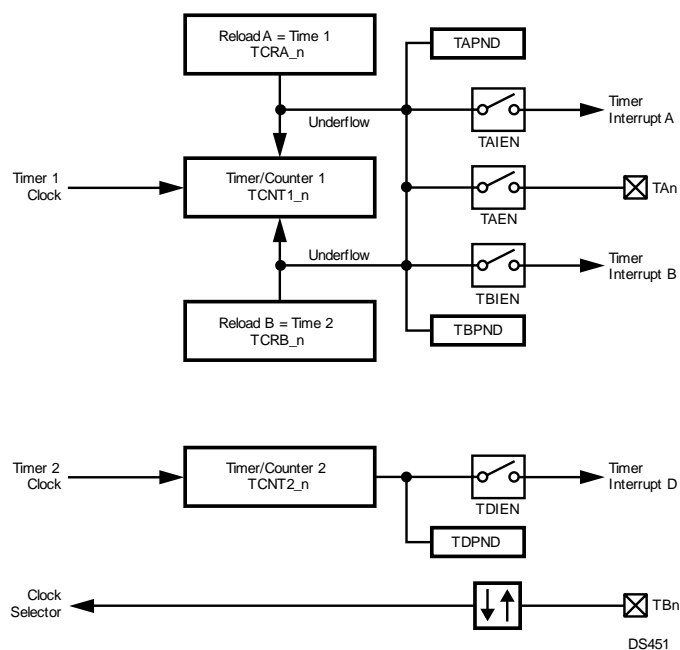
Figure 25-4. Processor-Independent PWM Mode
