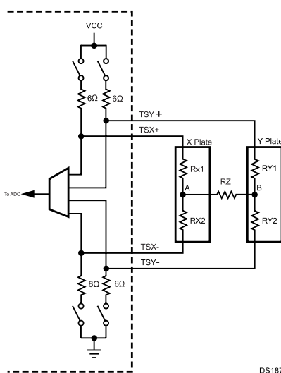
Figure 16-3. Touchscreen Driver Equivalent Circuit
