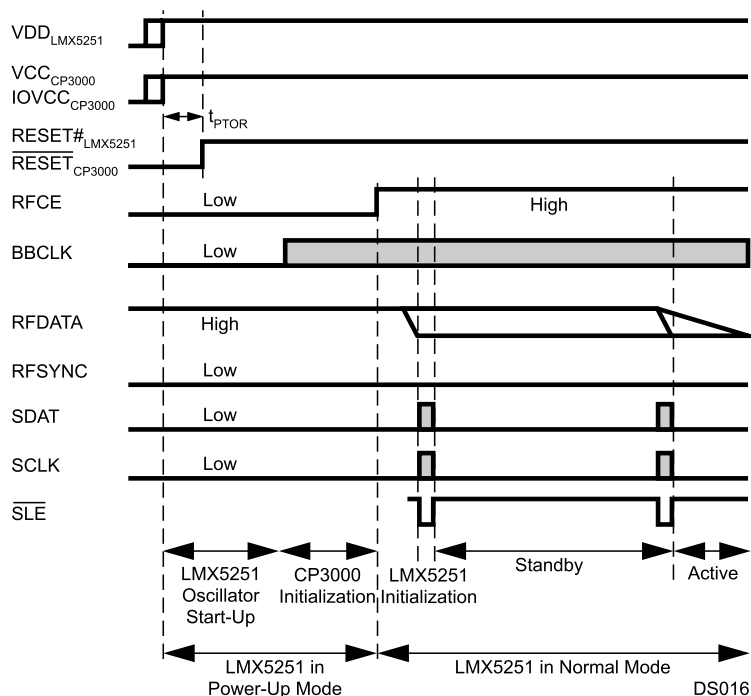
Figure 15-9. LMX5251 Power-Up Sequence
