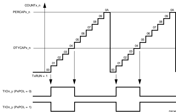
Figure 26-2. VTU PWM Generation
