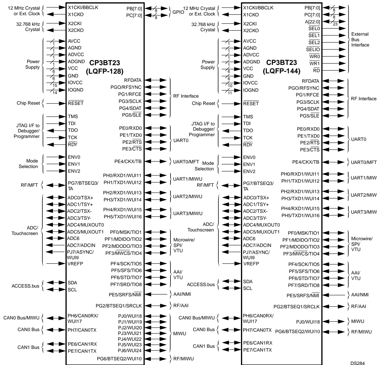
Figure 4-1. CP3BT23 Device Signals
