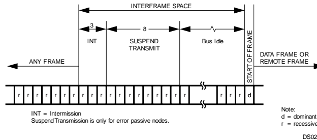
Figure 18-9. Interframe Space
