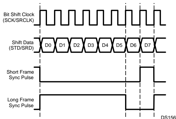
Figure 19-7. Short and Long Frame Sync Pulses
