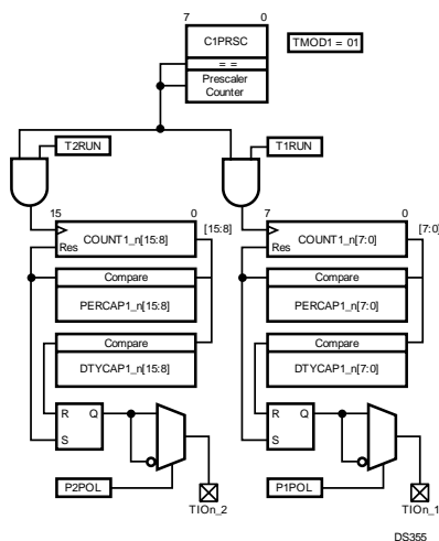
Figure 26-3. VTU Dual 8-Bit PWM Mode
