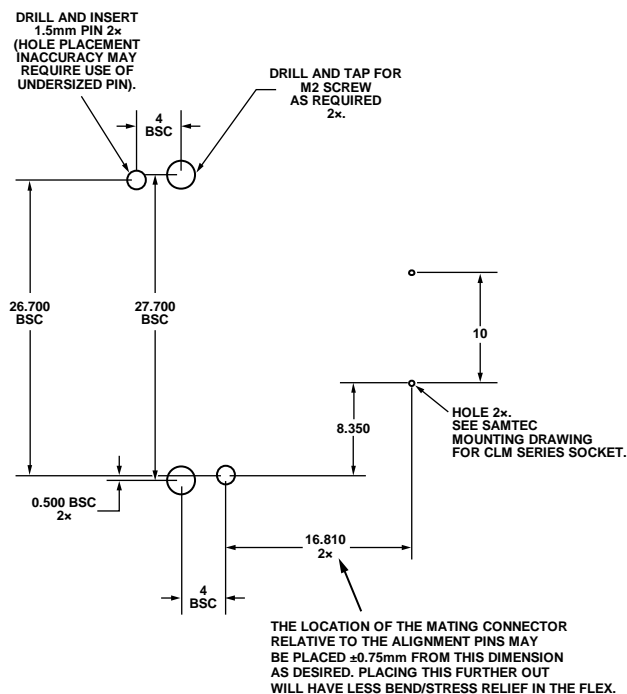
Figure 3. Suggested Mounting Hole Locations
