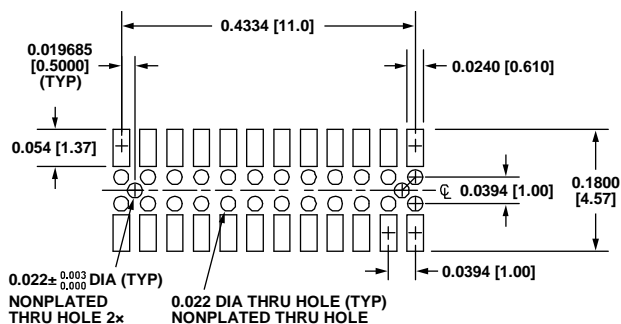
Figure 4. Suggested Layout and Mechanical Design for Mating Connector
