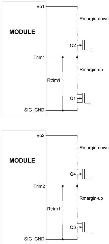
Figure 43. Circuit Configuration for margining Output voltage.
