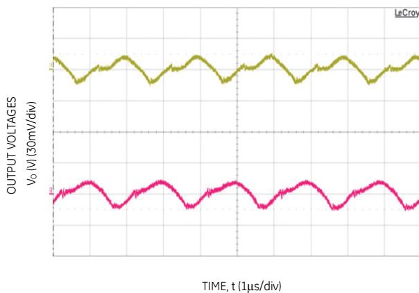
Figure 27. Typical output ripple and noise ( C_o = 2 \times 4.7\text{nF} + 2 \times 47\mu\text{F} ceramic, V_{IN} = 12\text{V} , I_o = I_{o1,max} , I_{o2,max} ).
