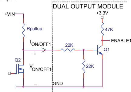
Figure 39. Circuit configuration for using positive On/Off logic.
