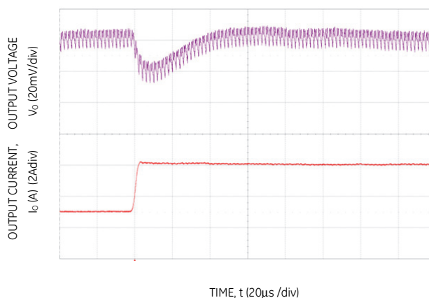
Figure 10. Transient Response to Dynamic Load Change on one output from 50% to 100% at 12Vin, C_{out} = 3 \times 47\mu\text{F} + 2 \times 330\mu\text{F} , C_{Tune} = 2700\text{pF} & R_{Tune} = 300\Omega
