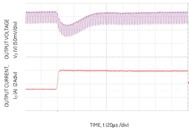
Figure 28 Transient Response to Dynamic Load Change on one output from 50% to 100% at 12V in , C_{out} = 2 \times 47\mu\text{F} + 1 \times 330\mu\text{F} , C_{Tune} = 1200\text{pF} & R_{Tune} = 300\Omega
