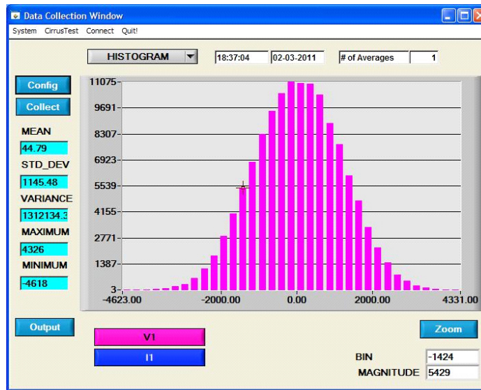
Figure 27. Histogram Analysis
