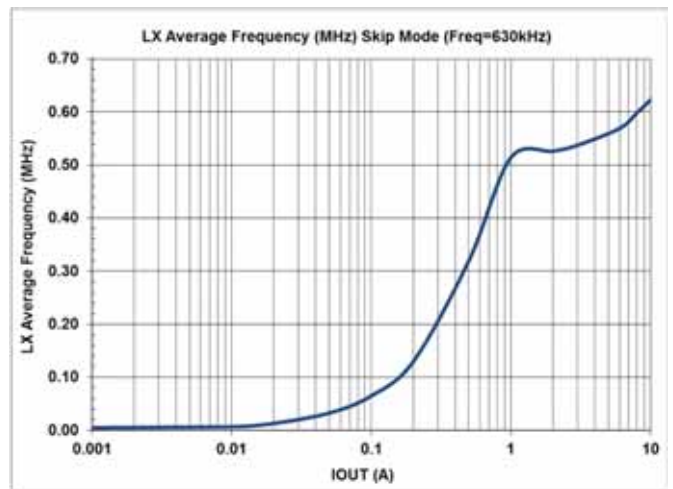
Frequency = 630 kHz
