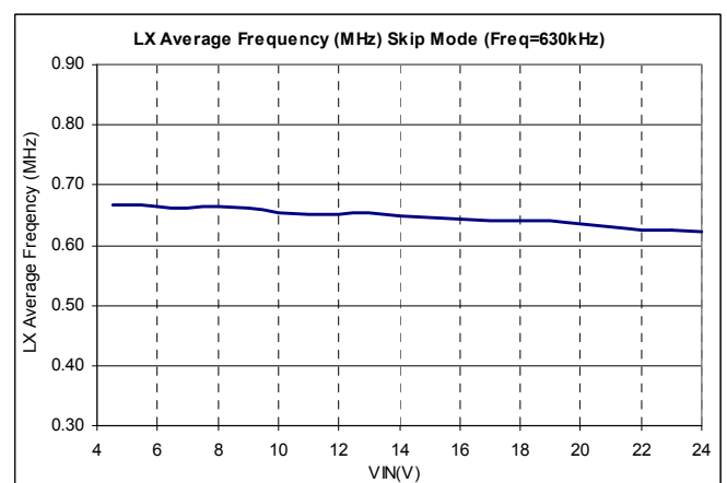
Frequency = 630 kHz
