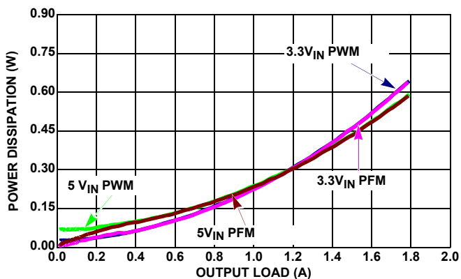
FIGURE 7. POWER DISSIPATION vs LOAD, 2.25MHz, 1.8V, CHANNEL 2
