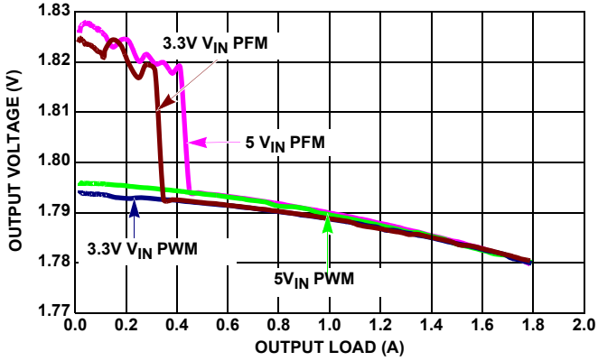
FIGURE 11. V_{OUT} REGULATION vs LOAD, 2.25MHz, 1.8V, CHANNEL 2
