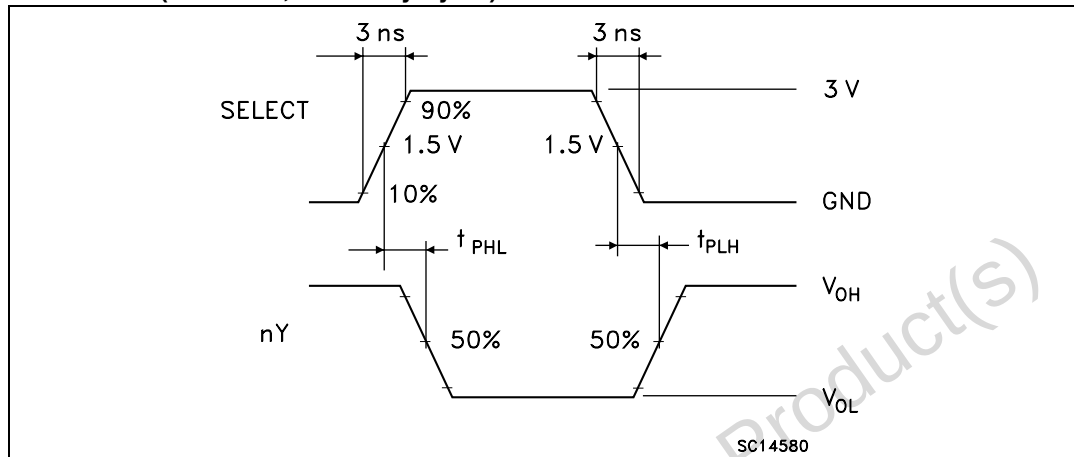
Figure 5. Waveform - propagation delays for inverting conditions ( f = 1 \text{ MHz} ; 50% duty cycle)
