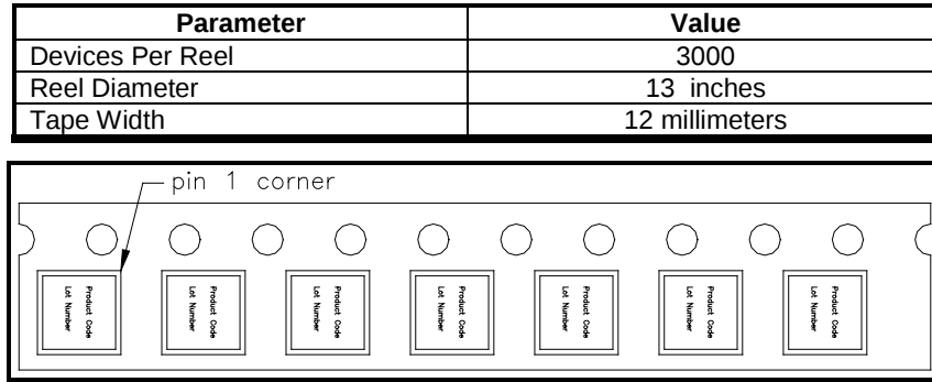
Figure 9: Detailed Tape and Reel Information (All diminensions in Millimeters)
