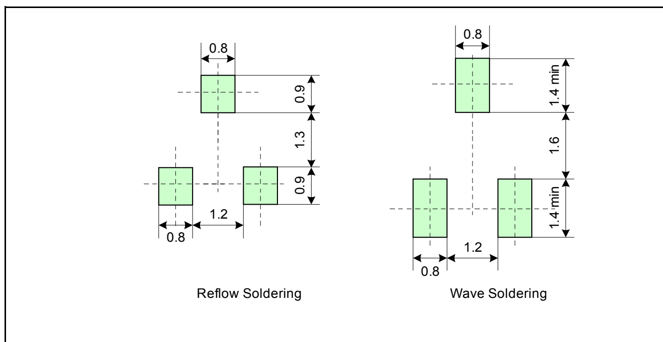
Figure 7 Footprint SC59 (SOT23 compatible)
