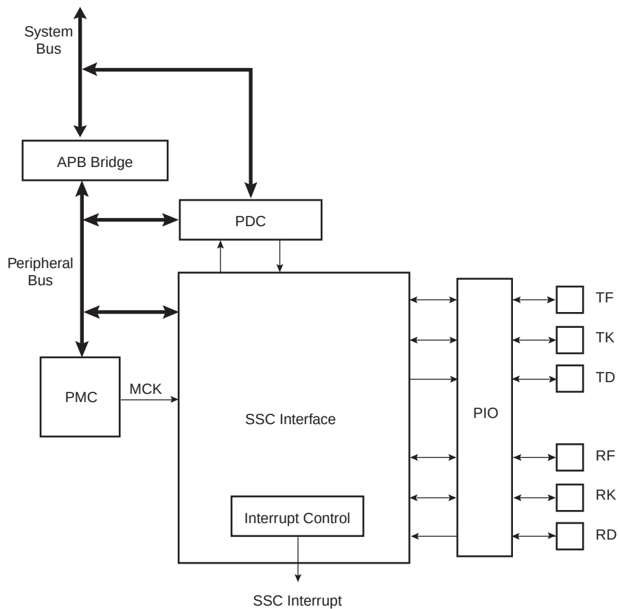
Figure 35-1. Block Diagram
