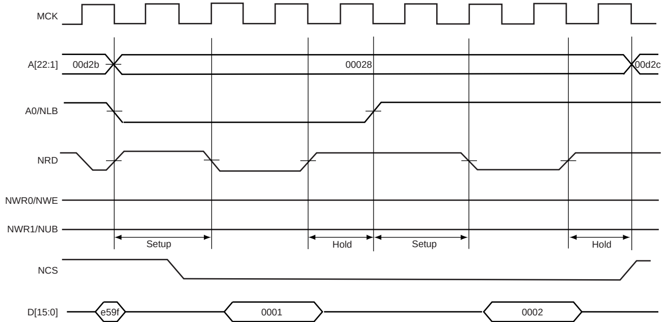
Figure 22-32. Read Accesses in Standard Read Protocol with Setup and Hold (1)
