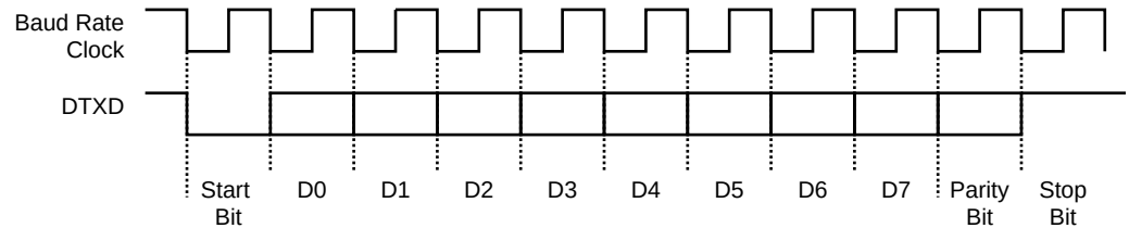
Figure 30-9. Character Transmission
