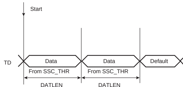
Figure 35-14. Transmit Frame Format in Continuous Mode
