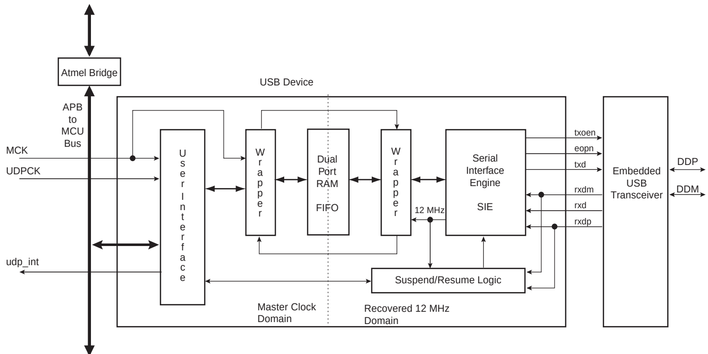
Figure 38-1. Block Diagram
