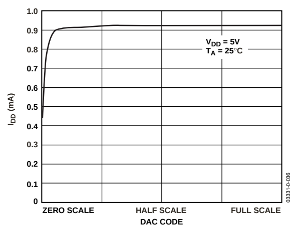
Figure 25. Supply Current vs. DAC Code
