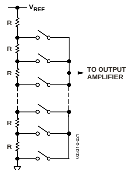
Figure 38. Resistor String
