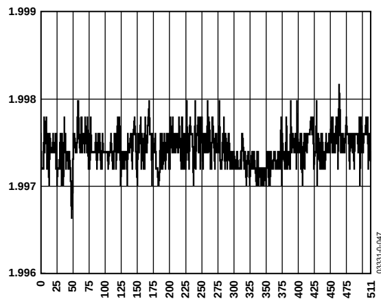
Figure 36. DAC-to-DAC Crosstalk
