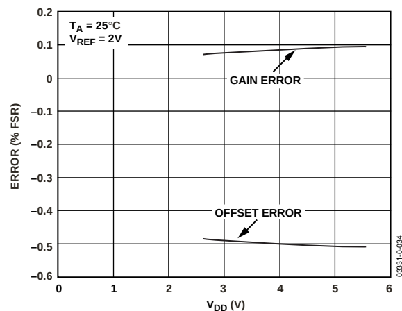
Figure 23. Offset Error and Gain Error vs. V_{DD}
