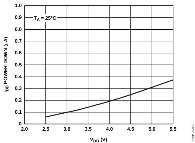
Figure 27. Power-Down Current vs. Supply Voltage
