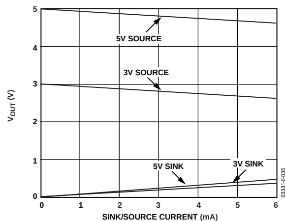
Figure 24. V_{OUT} Source and Sink Current Capability
