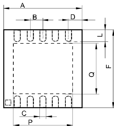
Figure 12.3 DFN-10 Package dimensions (bottom)
