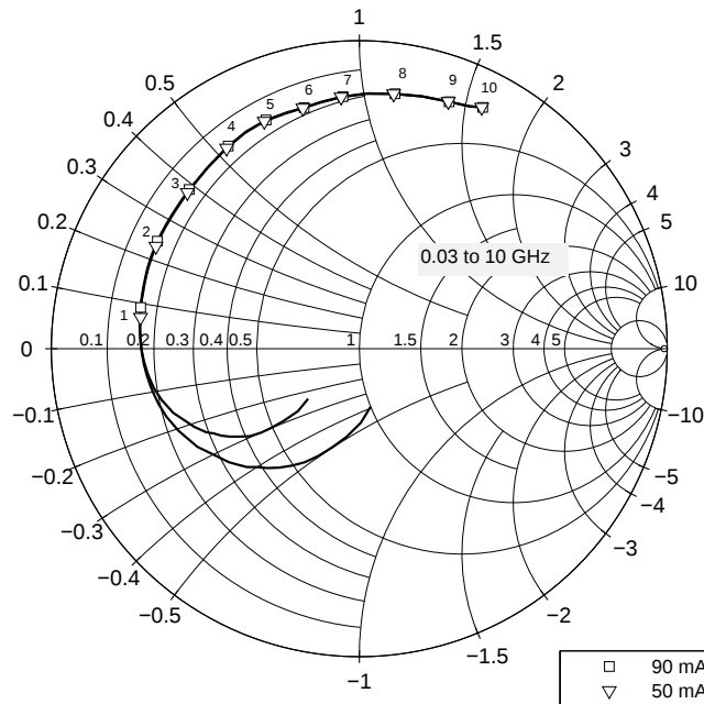
Figure 5-13 Input Matching S_{11} = f(f) , V_{CE} = 3\text{ V} , I_C = 50 / 90\text{ mA}
