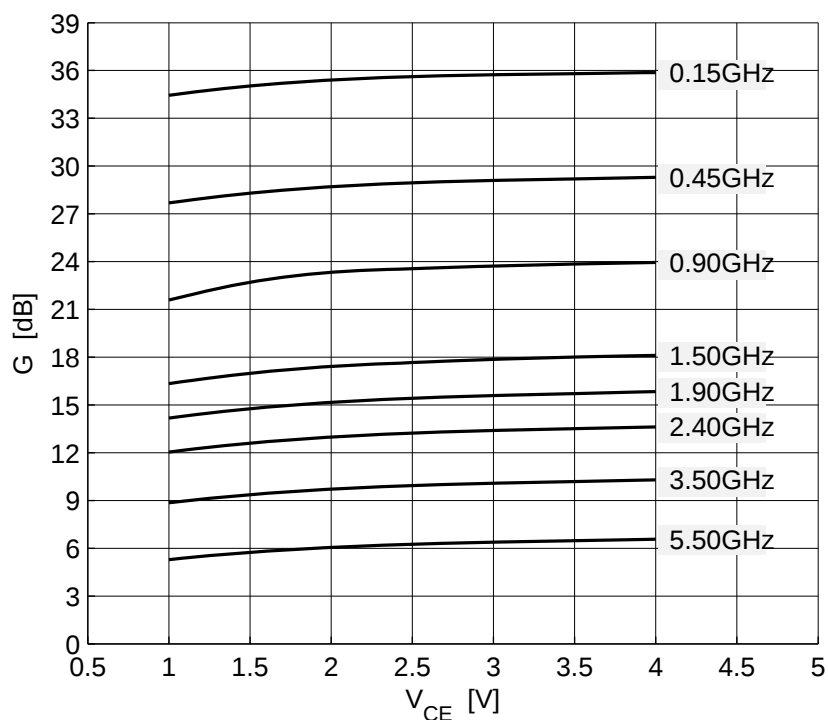
Figure 5-12 Maximum Power Gain G_{\max} = f(V_{CE}) , I_C = 90\text{ mA} , = Parameter in GHz
