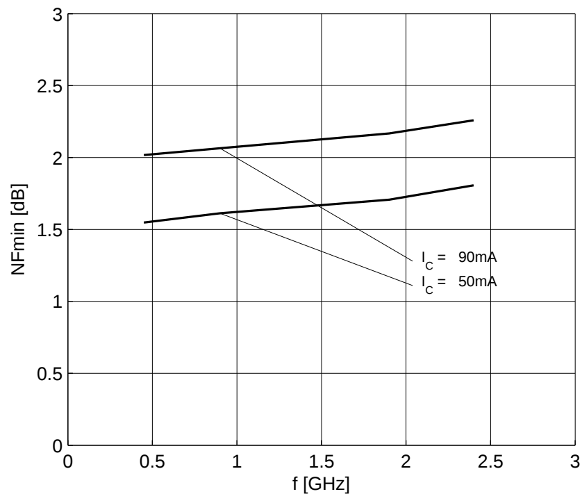
Figure 5-16 Noise Figure NF_{min} = f(f) , V_{CE} = 3\text{ V} , I_C = 50 / 90\text{ mA} , Z_S = Z_{opt}
