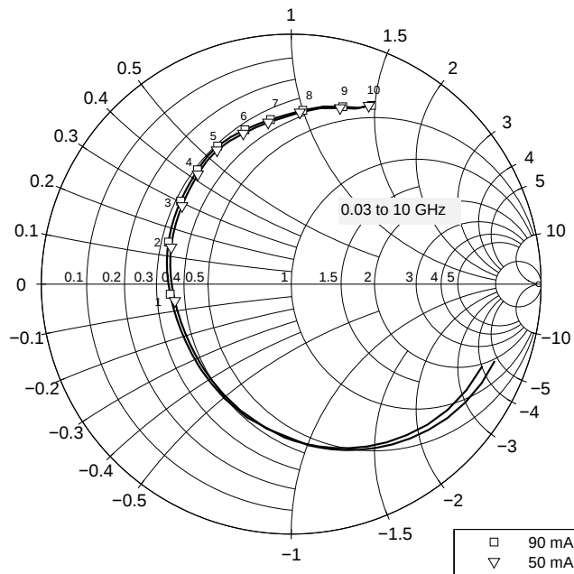
Figure 5-15 Output Matching S_{22} = f(f) , V_{CE} = 3\text{ V} , I_C = 50 / 90\text{ mA}
