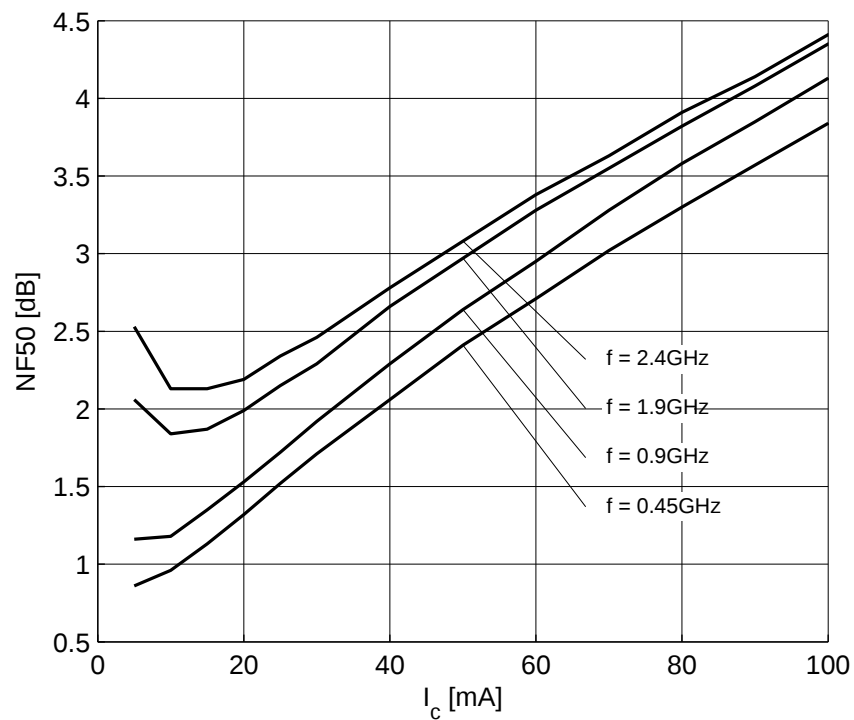
Figure 5-18 Noise Figure NF_{50} = f(I_C) , V_{CE} = 3\text{ V} , Z_S = 50\ \Omega = Parameter in GHz
