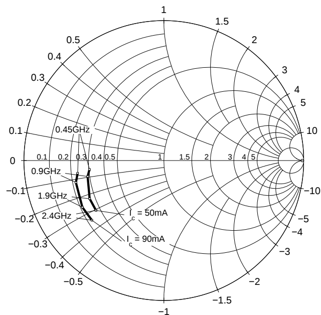
Figure 5-14 Source Impedance for Minimum Noise Figure = f(f) , V_{CE} = 3\text{ V} , I_C = 50 / 90\text{ mA}
