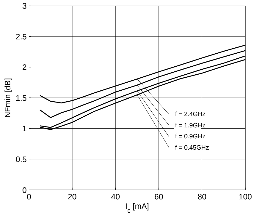
Figure 5-17 Noise Figure NF_{min} = f(I_C) , V_{CE} = 3\text{ V} , Z_S = Z_{opt} = Parameter in GHz
