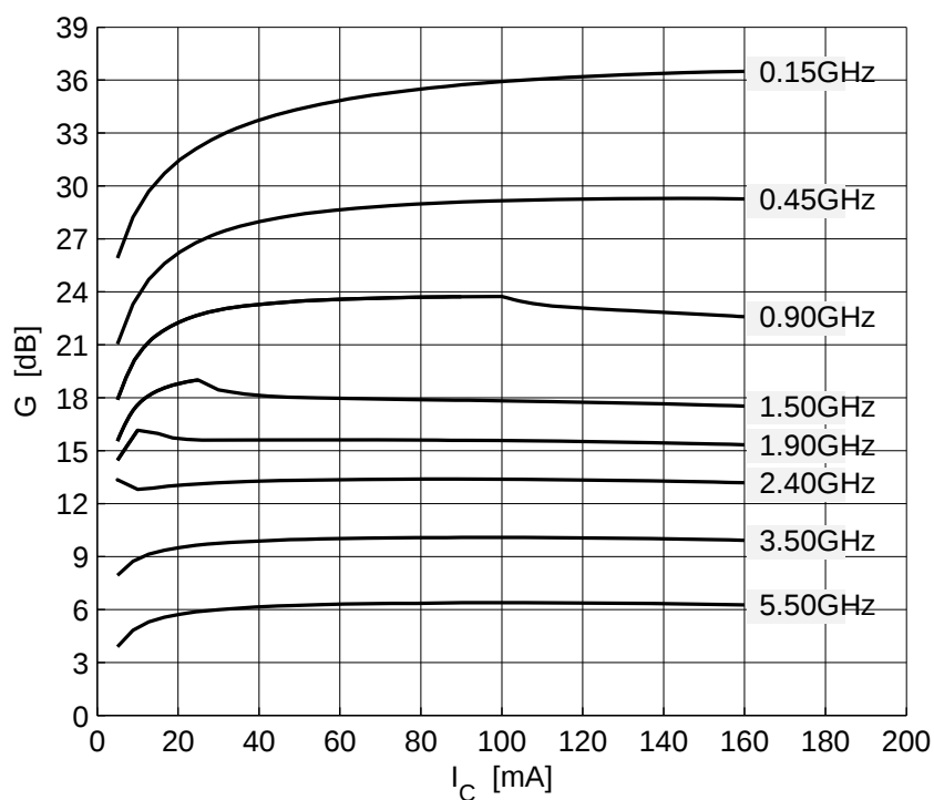
Figure 5-11 Maximum Power Gain G_{\max} = f(I_C) , V_{CE} = 3\text{ V} , = Parameter in GHz
