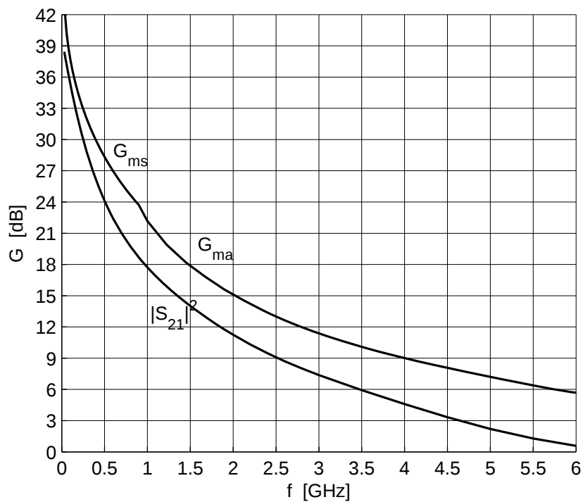
Figure 5-10 Gain G_{ma} , G_{ms} , |S_{21}|^2 = f(f) , V_{CE} = 3 V, I_C = 90 mA
