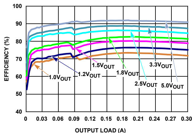
FIGURE 2. EFFICIENCY vs LOAD, PFM, V_{IN} = 12\text{V}
