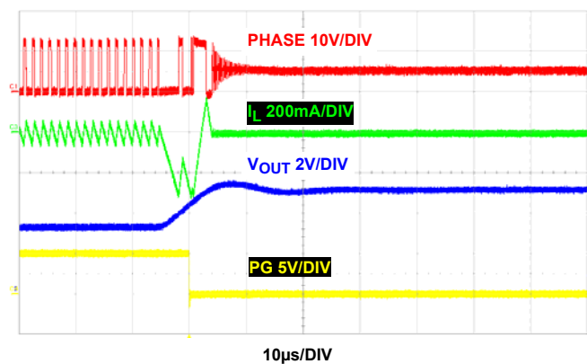
FIGURE 47. OVERVOLTAGE PROTECTION
