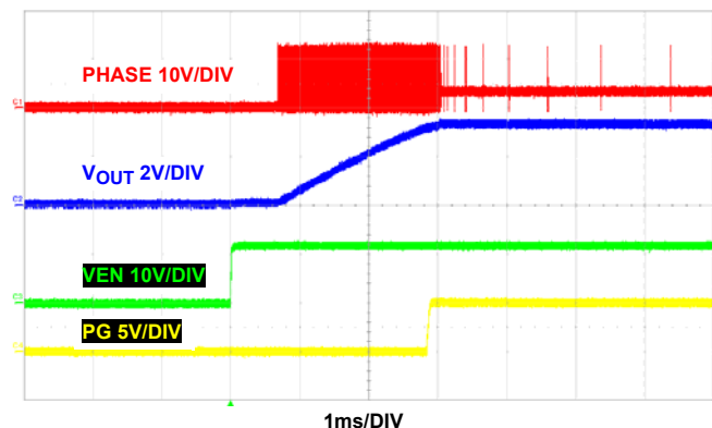
FIGURE 19. START-UP AT NO LOAD, PFM
