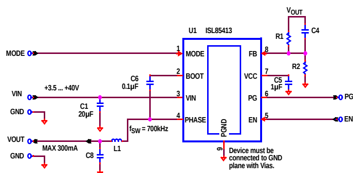
FIGURE 1. TYPICAL APPLICATION
