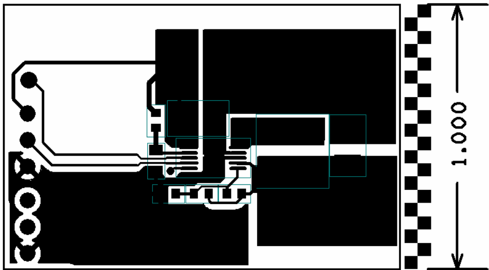
FIGURE 4: SP6651AEB PC LAYOUT TOP SIDE
