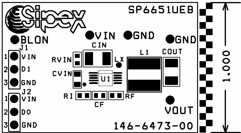
FIGURE 3: SP6651AEB COMPONENT PLACEMENT
