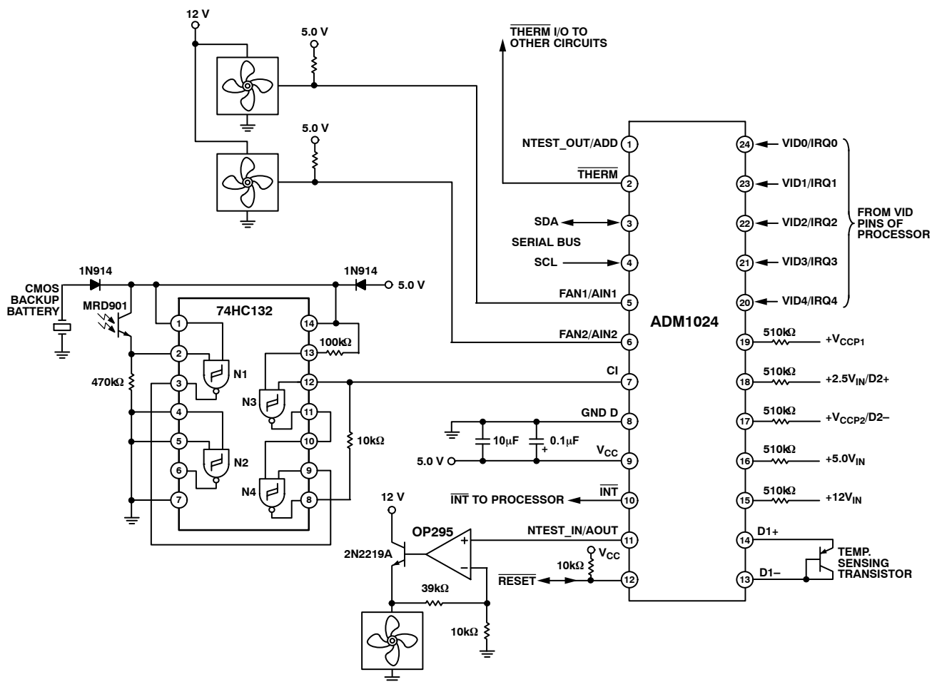
Figure 37. Application Circuit
