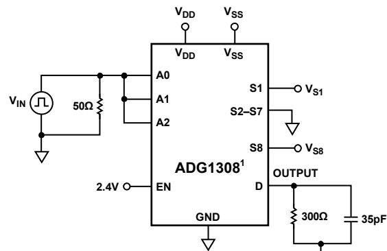
Figure 16. Address to Output Switching Times, t_{\text{TRANSITION}}
