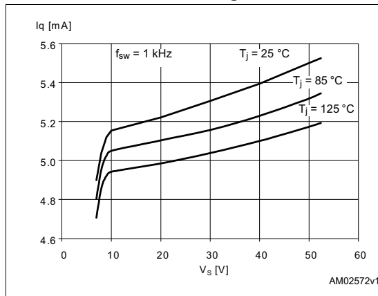
Figure 20. Typical quiescent current vs. supply voltage
