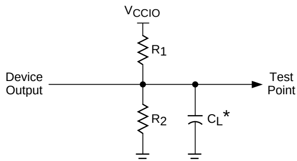
Figure 8. Test Load
