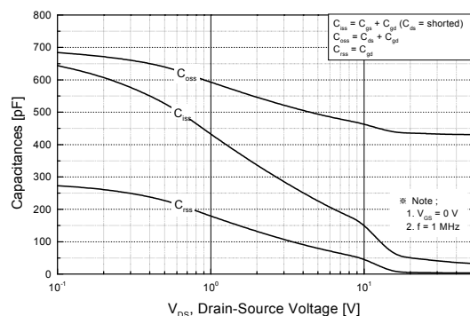
Figure 5. Capacitance Characteristics
