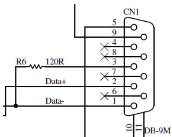
Figure 2.3 USB-COM485-PLUS1 Termination resistor
