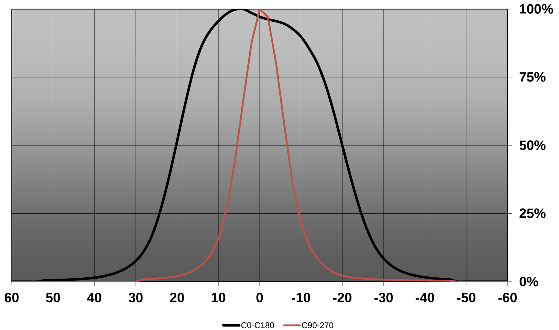
Relative intensity of CA12012_LAURA-O-PIN_(Oslon_Square_PC)
