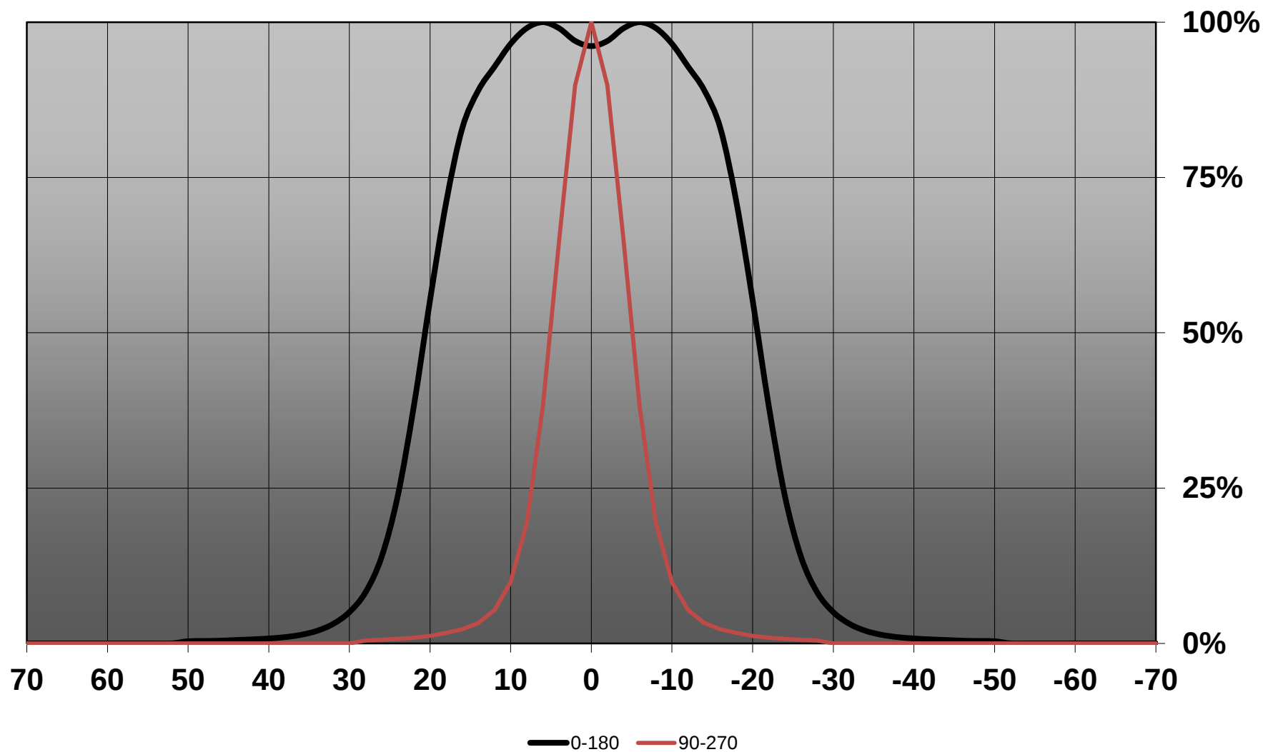
Relative intensity of CA12012_LAURA-O-PIN_(XP-E2)
