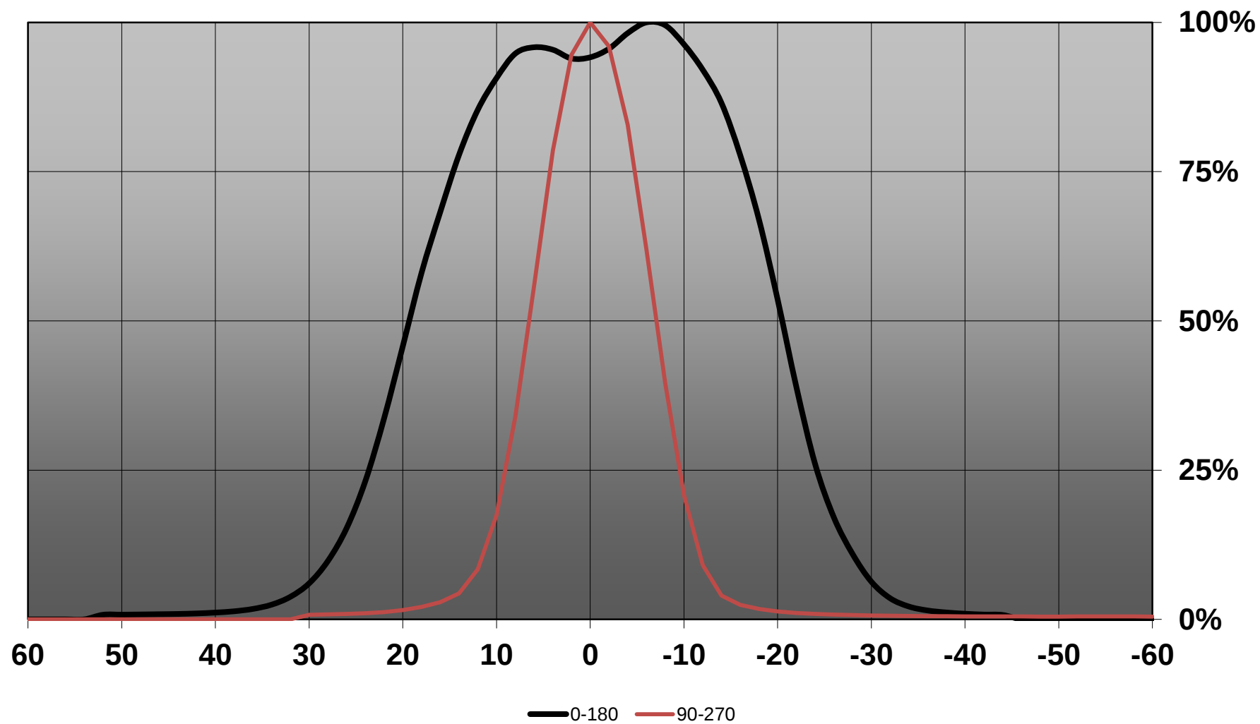
Relative intensity of CA12012_LAURA-O-PIN_(SFH4725S)
