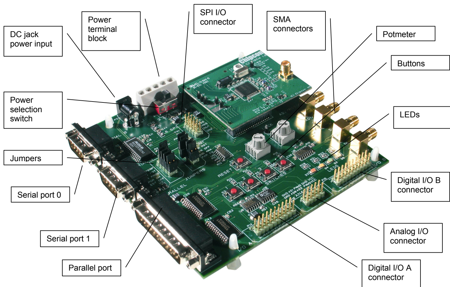
Figure 5: CC1010EB Evaluation Board (with CC1010EM plugged in)
