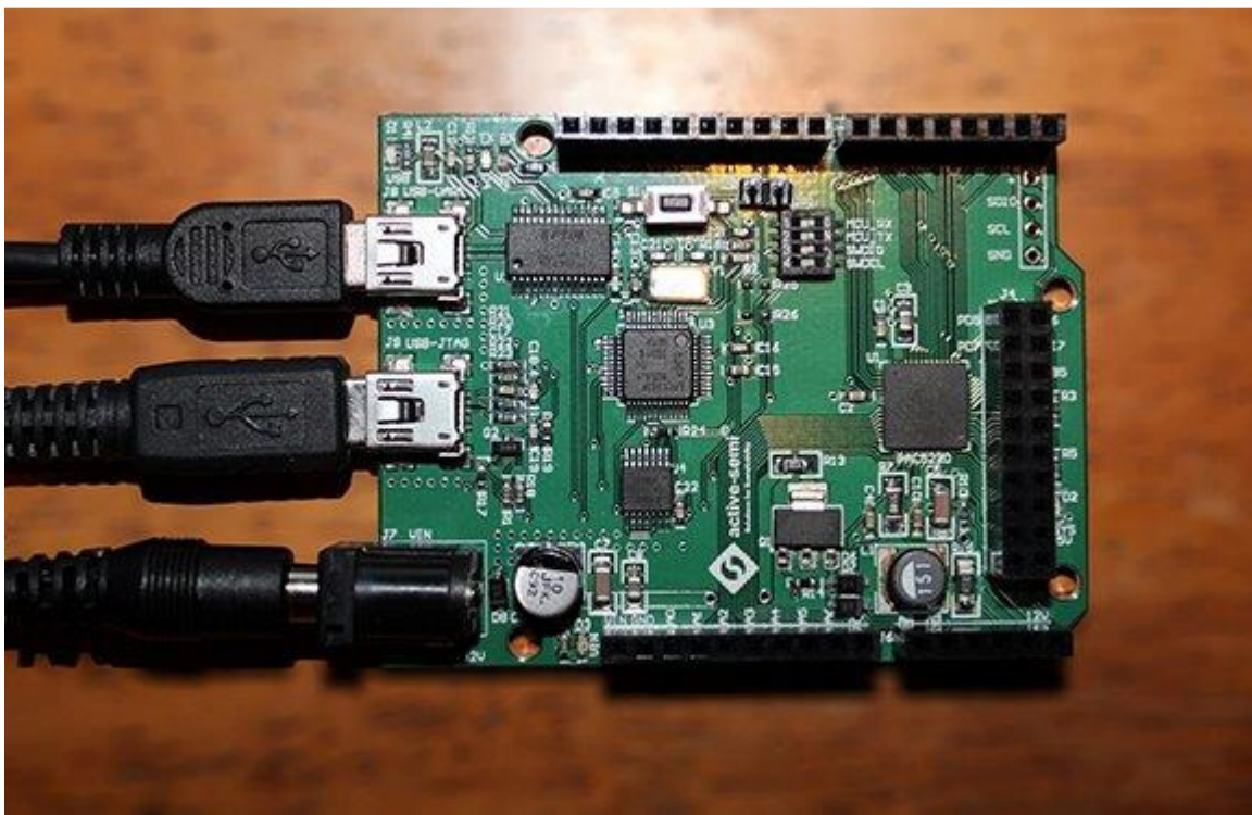
Figure 7:HYDRA-X10 Connections
