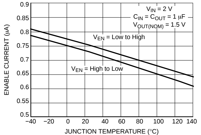
Figure 50. Enable Threshold Voltage vs. Temperature
