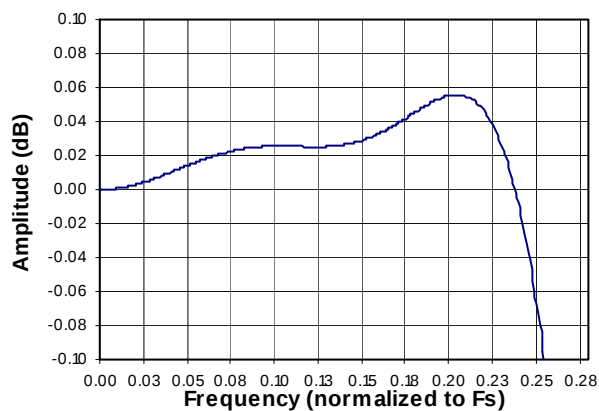
Figure 12. Quad-Speed Mode Passband Ripple
