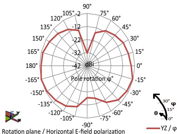
Fig. 5 - VJ5301M868MXBSR YZ Radiation Pattern
