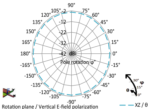
Fig. 6 - VJ5301M868MXBSR XZ Radiation Pattern
