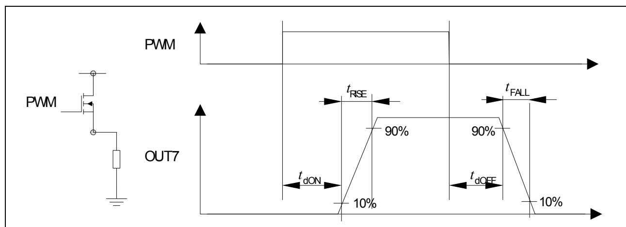
Figure 15 Timing OUT 7
