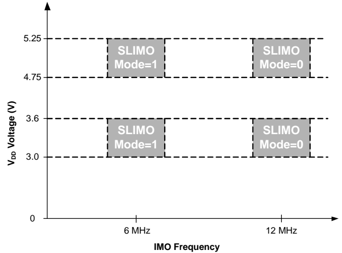
Figure 4. IMO Frequency Trim Options
