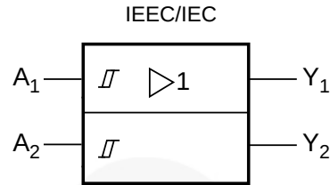
Figure 1. Logic Symbol
