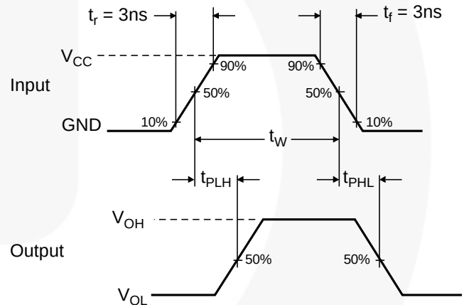
Figure 6. AC Waveforms
