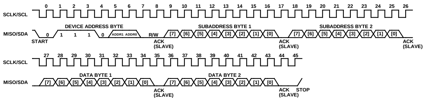
Figure 27. I 2 C Slave Single Word Write Operation (Two Bytes)
