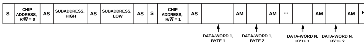
Figure 33. Simplified Burst Mode I 2 C Read Sequence
