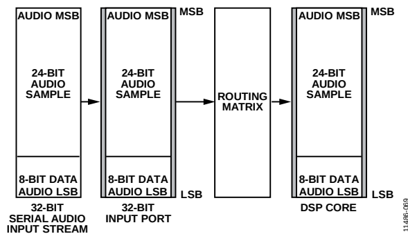
Figure 66. 32-Bit Serial Input Example
