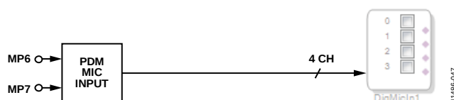
Figure 44. PDM Microphone Input Mapping to DSP in SigmaStudio
