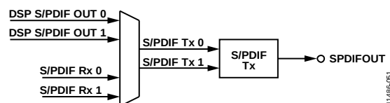
Figure 48. S/PDIF Transmitter Source Selection
