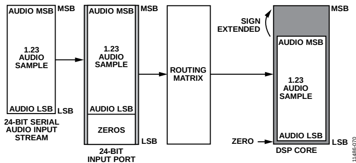
Figure 68. 24-Bit Serial Input Example
