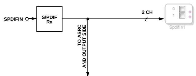
Figure 45. S/PDIF Receiver Direct Input Mapping to DSP in SigmaStudio
