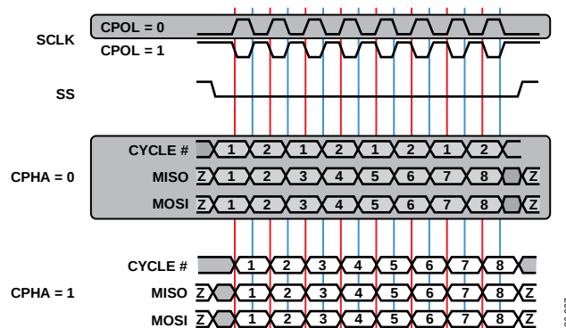
Figure 35. Clock Polarity and Phase for SPI Slave Port
