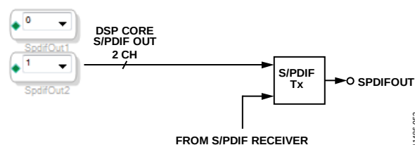
Figure 49. DSP to S/PDIF Transmitter Output Mapping in SigmaStudio
