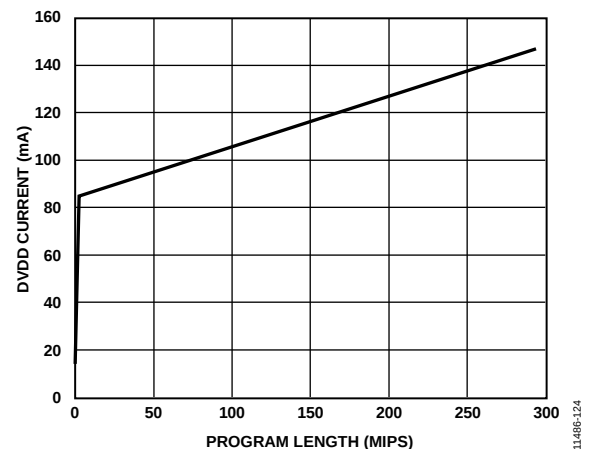
Figure 25. ADAU1452 Typical DVDD Current Draw vs. Program MIPS at an Ambient Temperature of 25°C and a Sample Rate of 48 kHz
