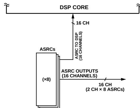
Figure 58. ASRC Outputs
