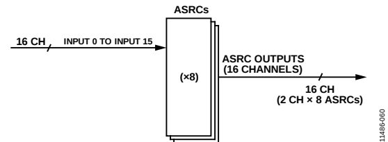
Figure 57. Example ASRC Routing, Bypassing DSP Core
