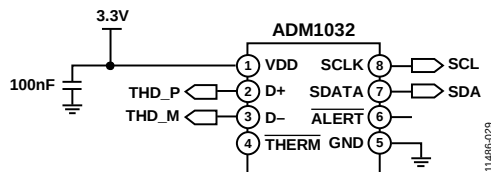
Figure 26. Example External Temperature Sensor Circuit
