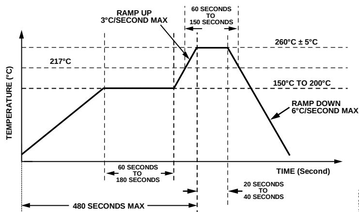
Figure 89. Soldering Profile
