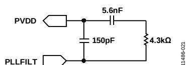
Figure 17. PLL Filter
