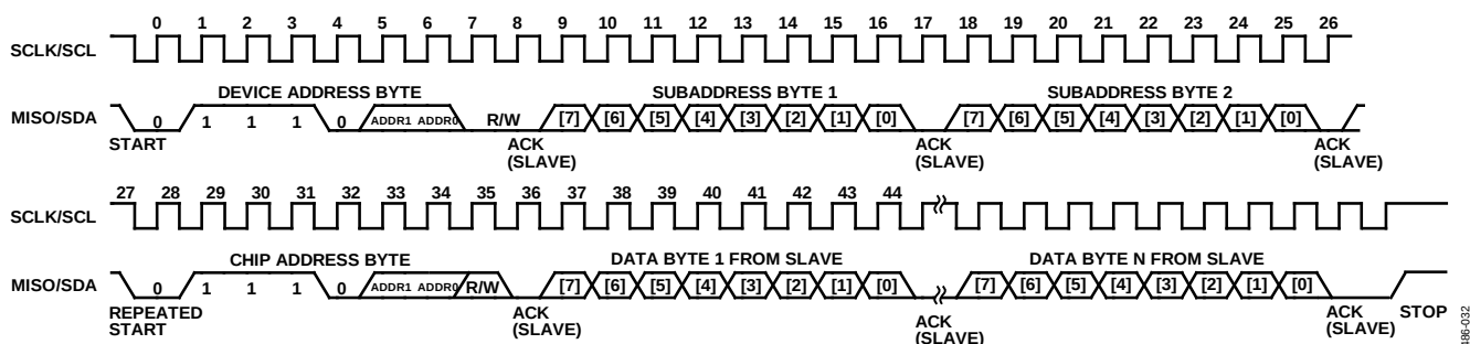
Figure 29. I 2 C Slave Burst Mode Read Operation (N Bytes)
