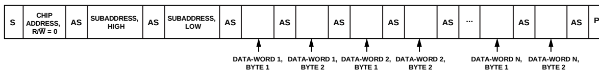
Figure 31. Simplified Burst Mode I 2 C Write Sequence
