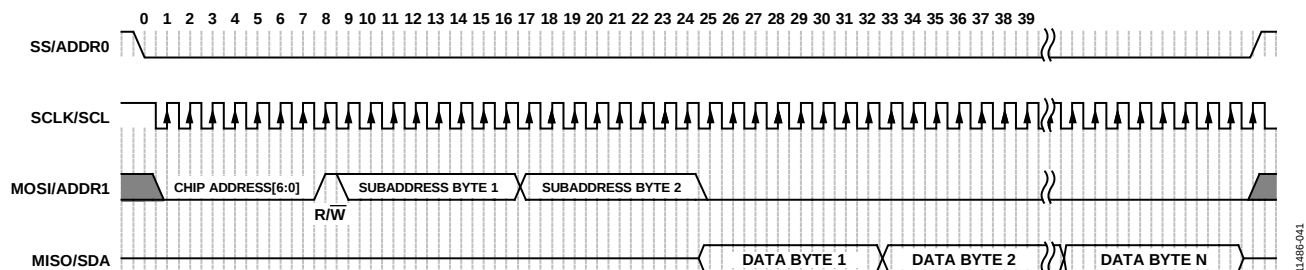
Figure 38. SPI Slave Read Clocking (Burst Read Mode, N Bytes)
