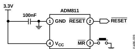
Figure 24. Example Manual Reset Generation Circuit
