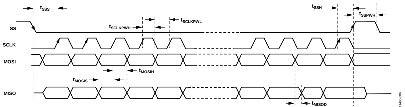
Figure 9. SPI Slave Port Timing Specifications
