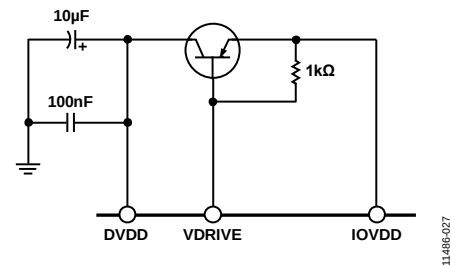
Figure 22. External Components Required for Voltage Regulator Circuit
