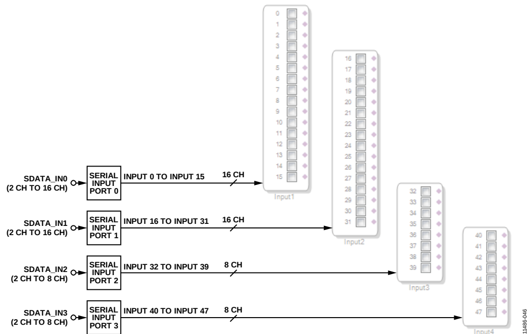
Figure 43. Serial Port Audio Input Mapping to DSP in SigmaStudio
