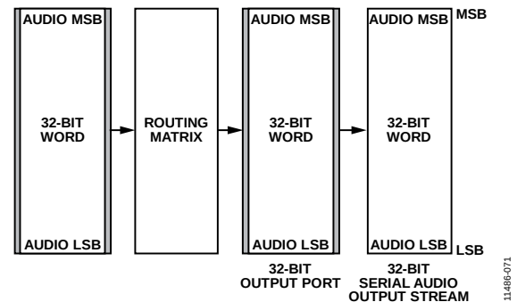
Figure 67. 32-Bit Serial Output Example
