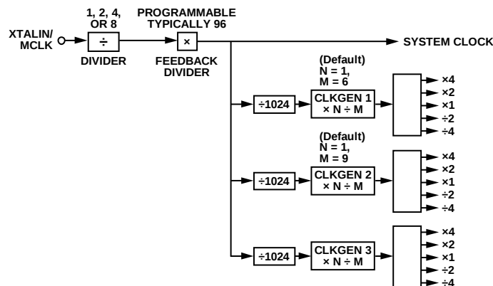
Figure 18. PLL and Clock Generators Block Diagram
