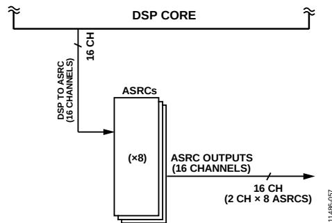
Figure 54. Example ASRC Routing for Asynchronous Serial Output from the DSP Core
