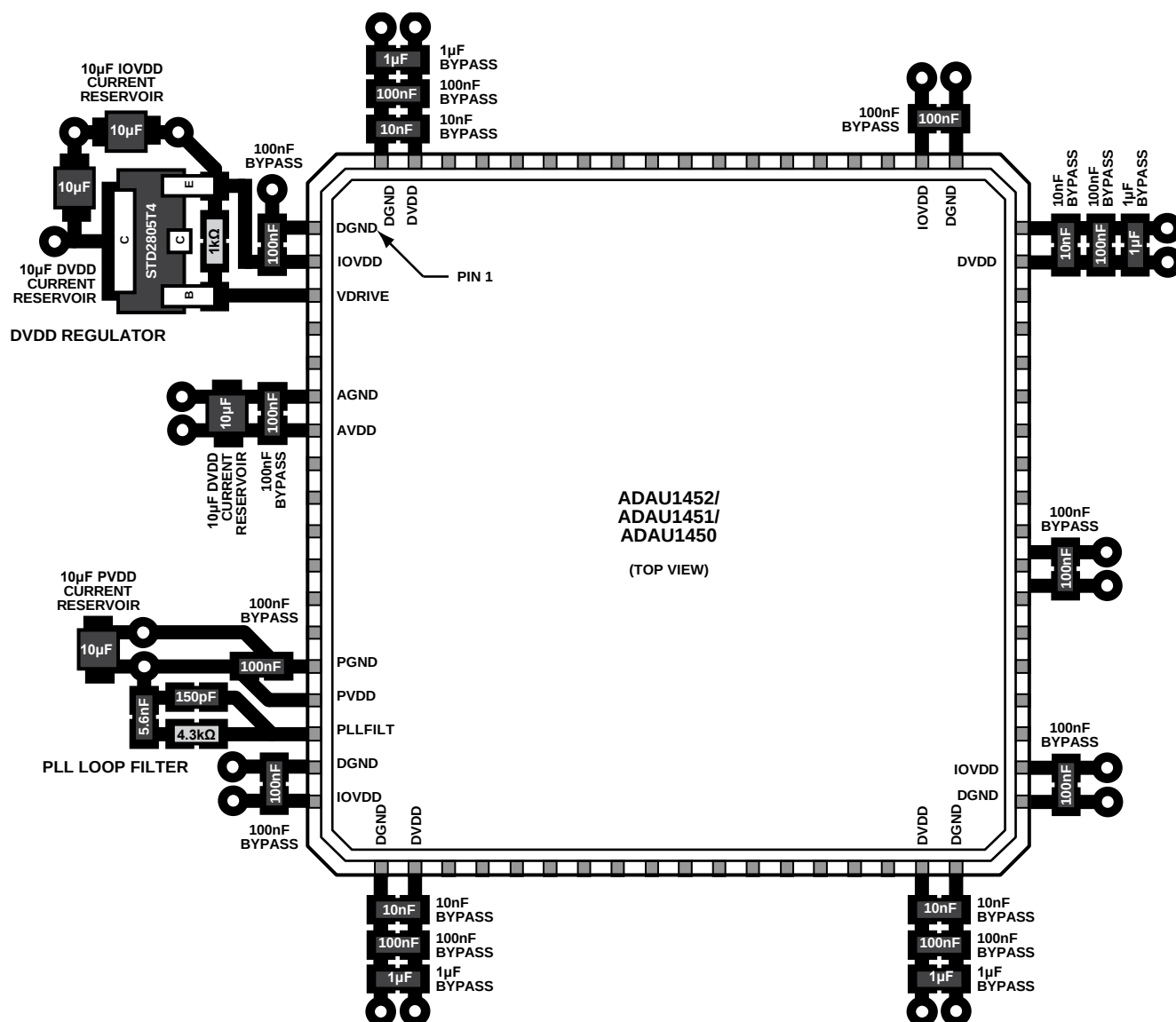
Figure 88. Supporting Component Placement and Layout
