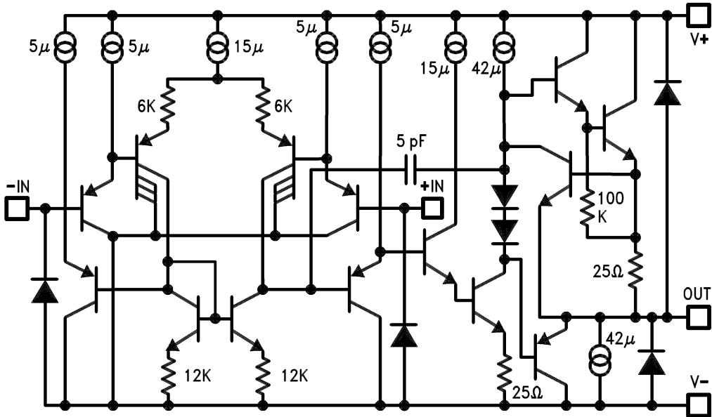
Figure 4. Op Amp
