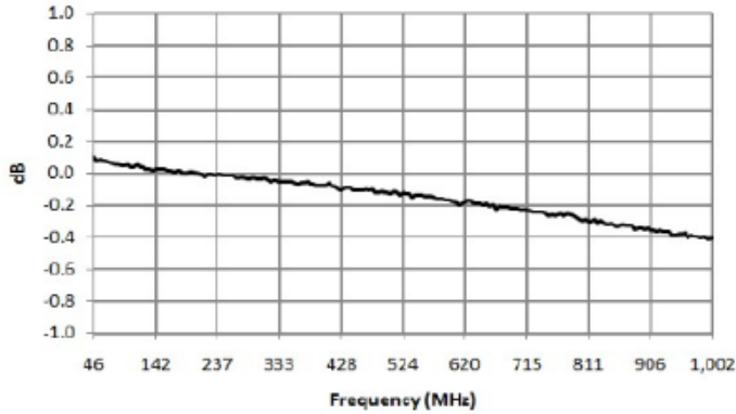
MABA-010245-CT1160 insertion_loss_pin_4_3
