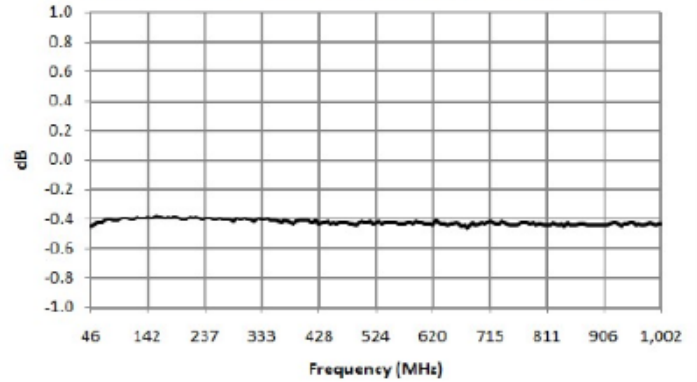
MABA-010245-CT1160 insertion_loss_pin_4_1
