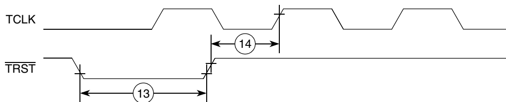
Figure 27. \overline{TRST} Timing Debug AC Timing Specifications
