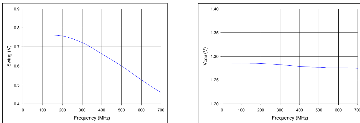
Figure 3. 2.5-V Supply and Termination to V_{DD} –2 V, Minimum V_{DD} and Maximum T_A
