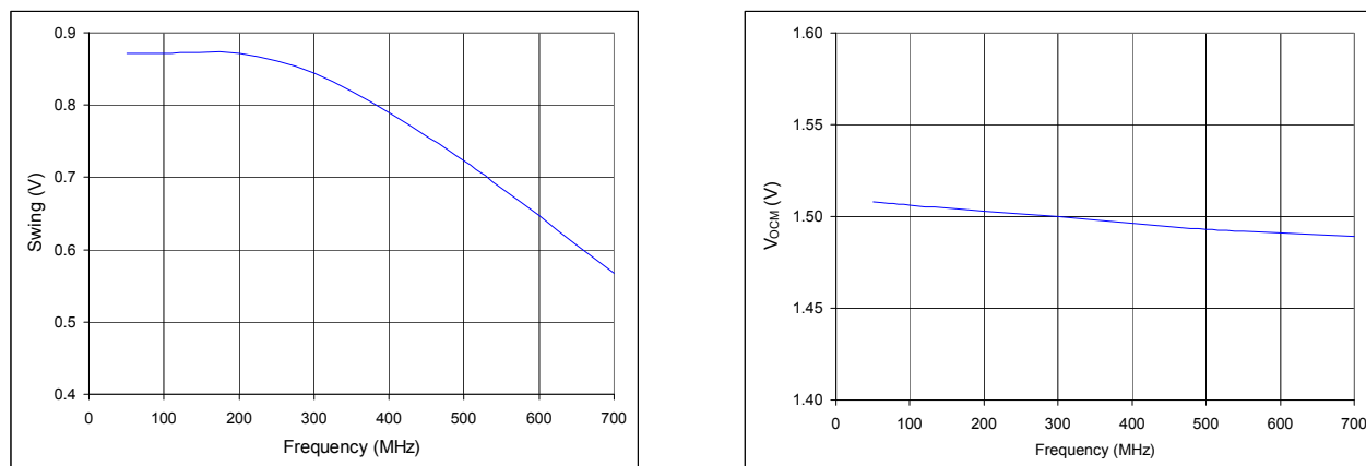
Figure 4. 3.3-V Supply and Termination to V_{DD} –2 V, Minimum V_{DD} and Maximum T_A
