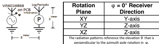
Fig. 3 - VJ5601M868 PCB Mounting and Coordinate Directions
