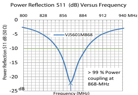
Fig. 2 - VJ5601M868 Tuned to 868 MHz with > 99 % Power Coupled
