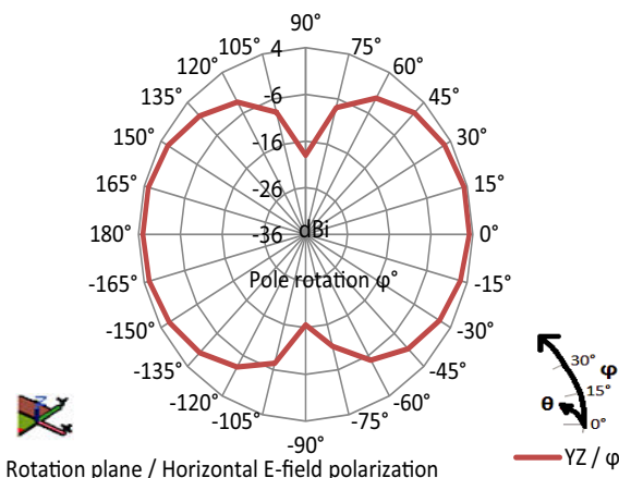
Fig. 5 - VJ5601M868MXBSR YZ Radiation Pattern
