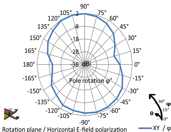
Fig. 4 - VJ5601M868MXBSR XY Radiation Pattern
