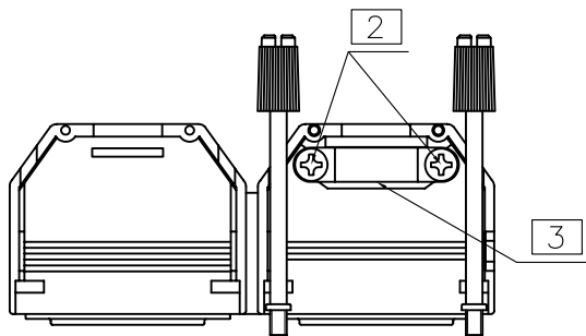
Drawing for sub-assembly L17DPPK15JS
