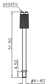
1 thumb screw
