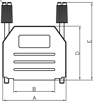
Drawing for sub-assembly L17DPPK15JS
