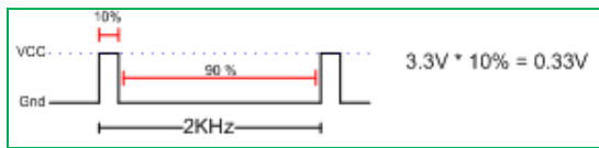
Figure 1. 10% Duty Cycle
