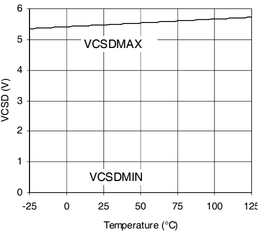
VCSDMIN,MAX vs TEMP (IR2161)
