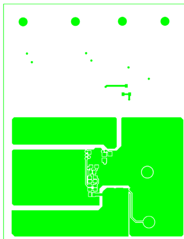
FIGURE 6. BOTTOM LAYER
